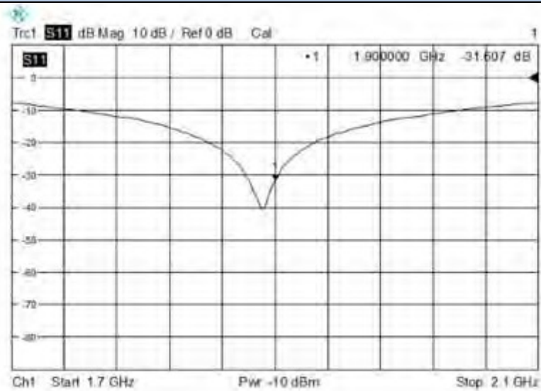
Return loss
