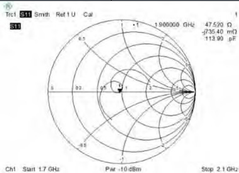
Impedance
