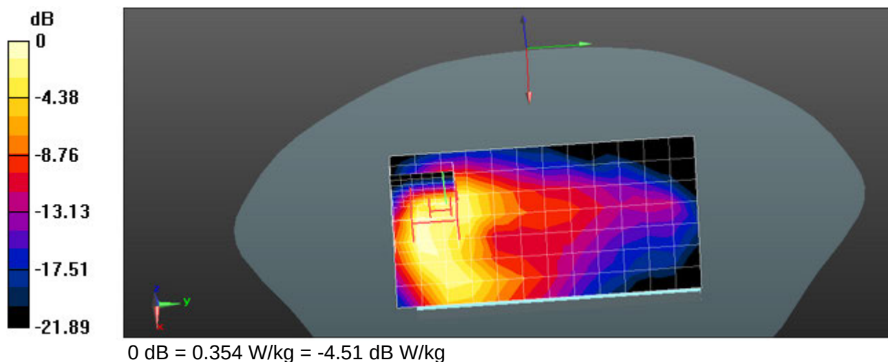
Figure 8: Body, Rear Side, 802.11b Channel 6
