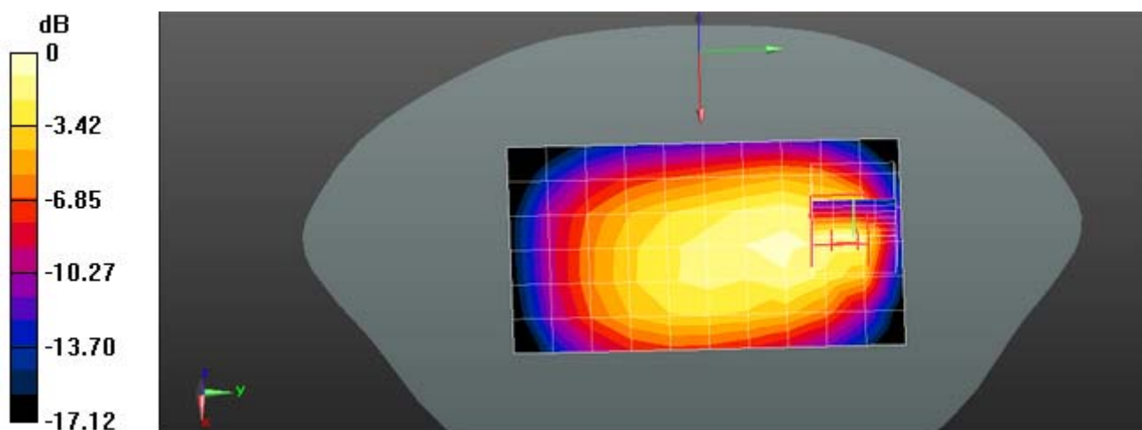
Figure 2 : Body Rear Side, GSM 850 GPRS (2Txslots) Channel 190
