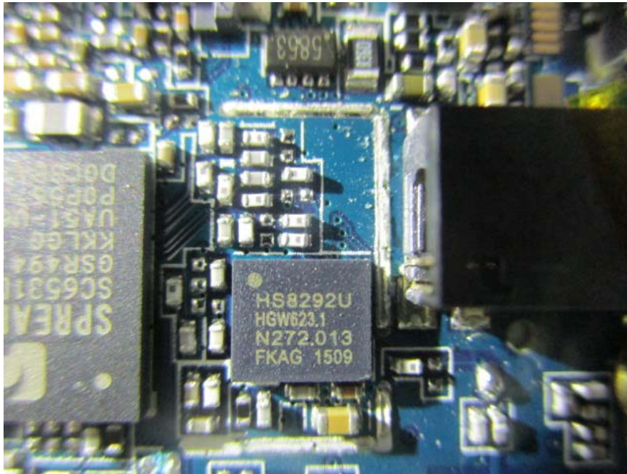
EUT –GSM RFPA Chip View
