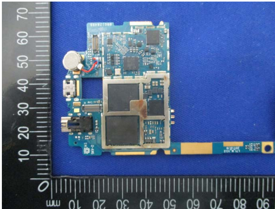
EUT –Main Board Bottom Unshiled View
