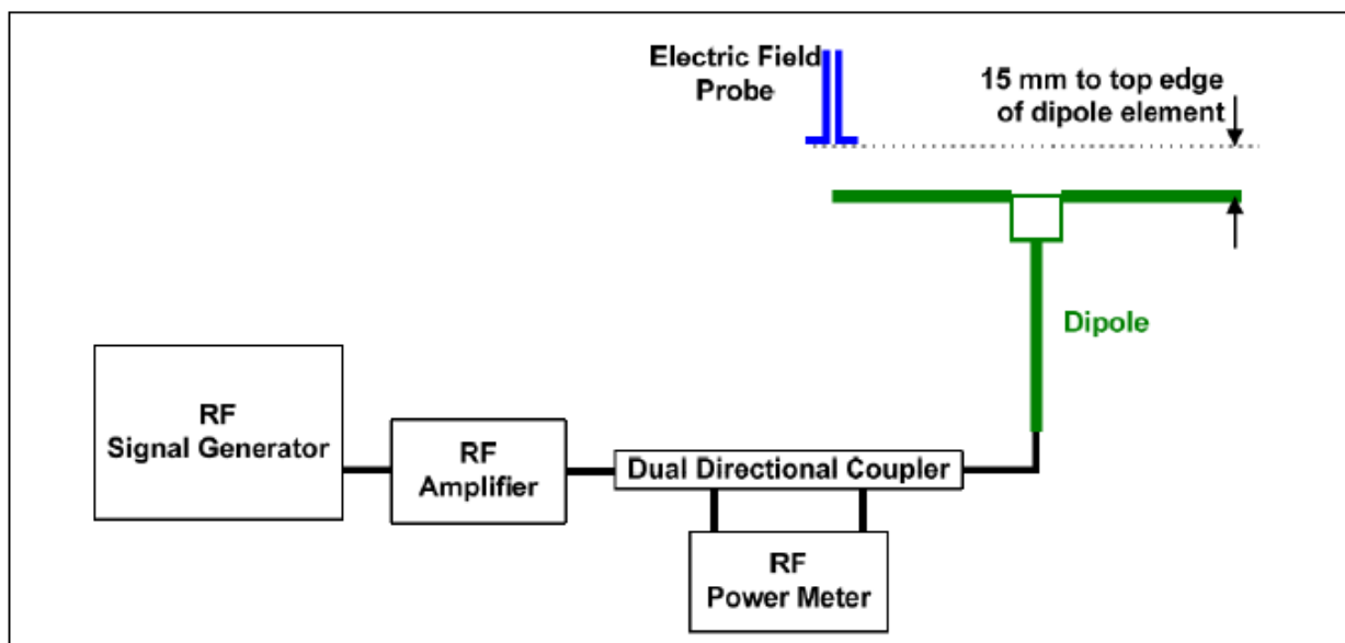
Setup diagram
