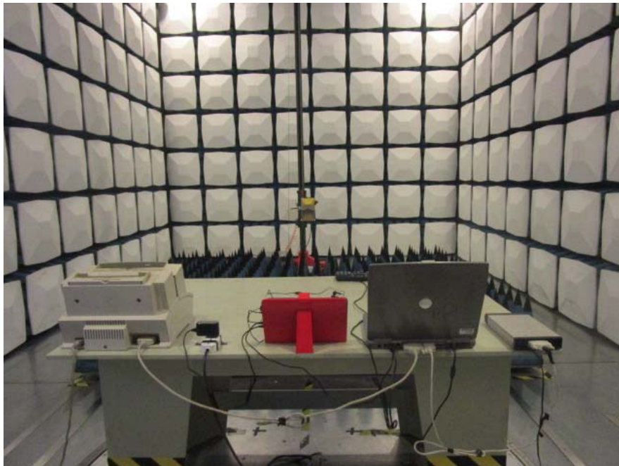
Radiated Emission –Rear View (Above 1 GHz) (Charging&Downloading)
