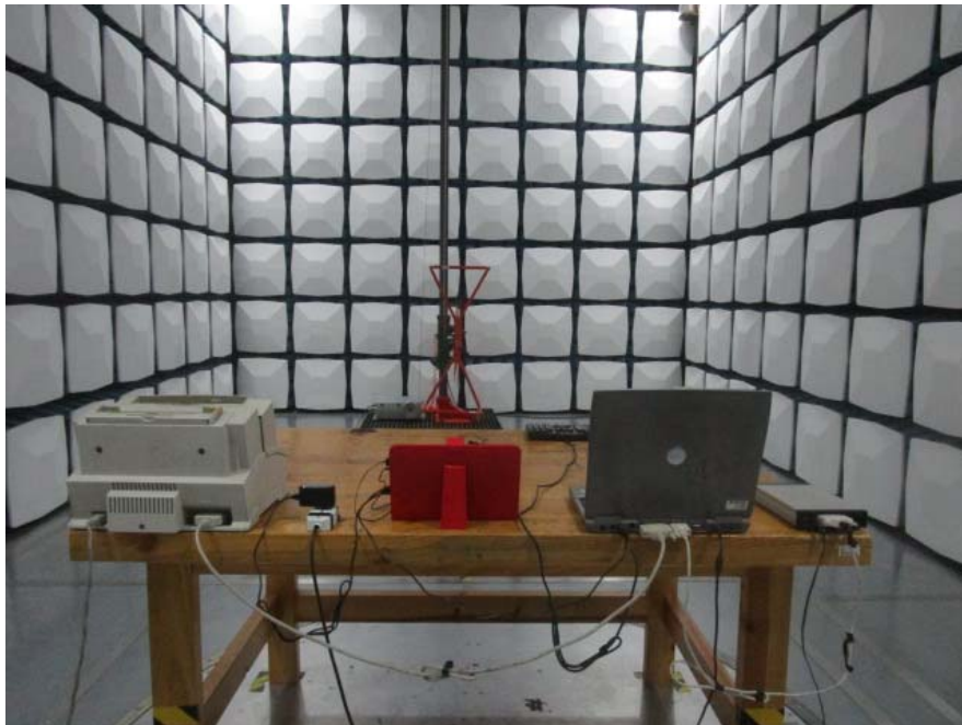
Radiated Emissions –Rear View (Below 1GHz) (Charging&Downloading)
