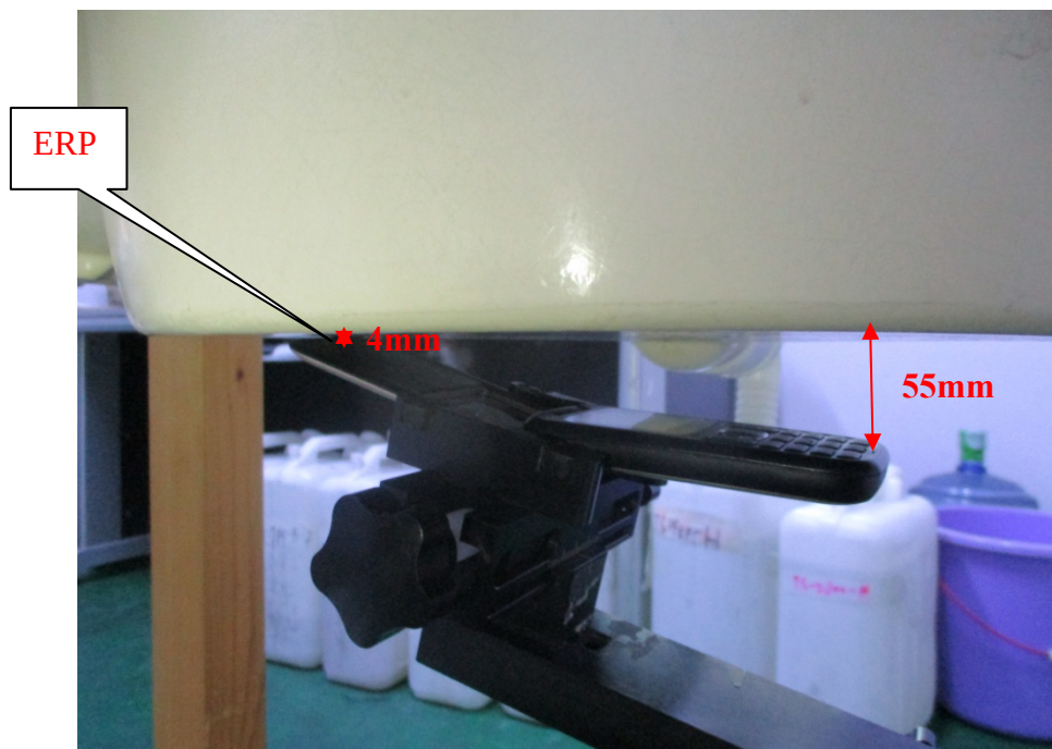
Head Flat Setup Photo
