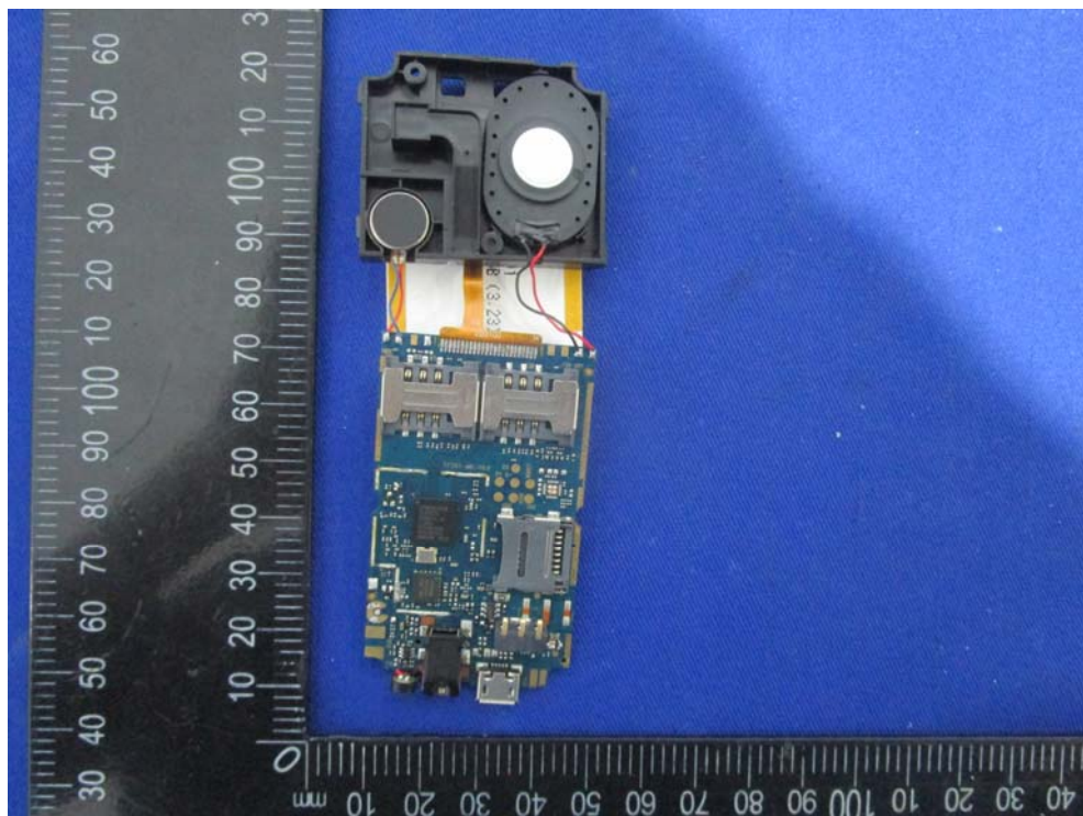
2G Antenna
