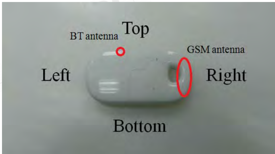
Antenna position photo
