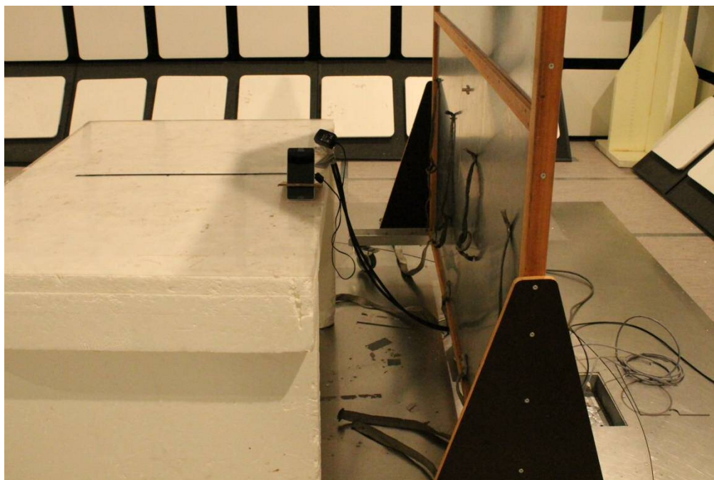
Photograph 3. Conducted emissions.
