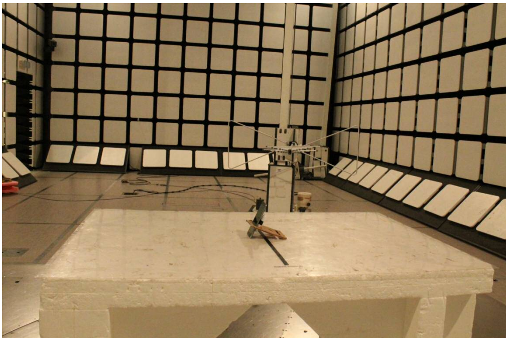
Photograph 2. Radiated Spurious Emissions 30 – 1000 MHz
