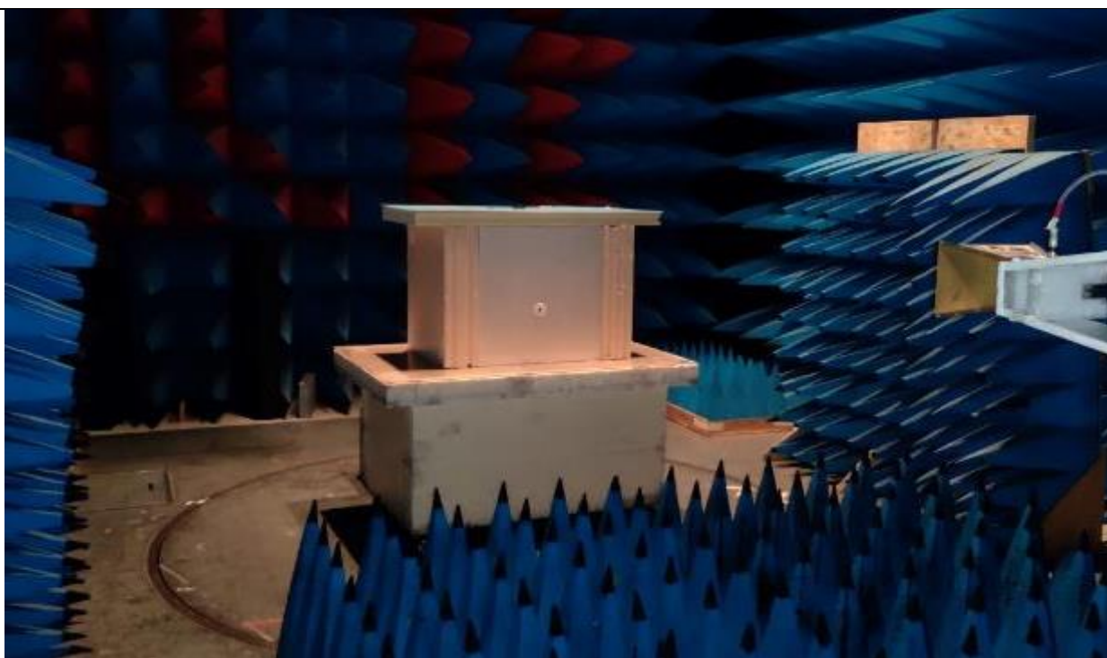
Photograph for Field strength of fundamental & Field strength of harmonics
