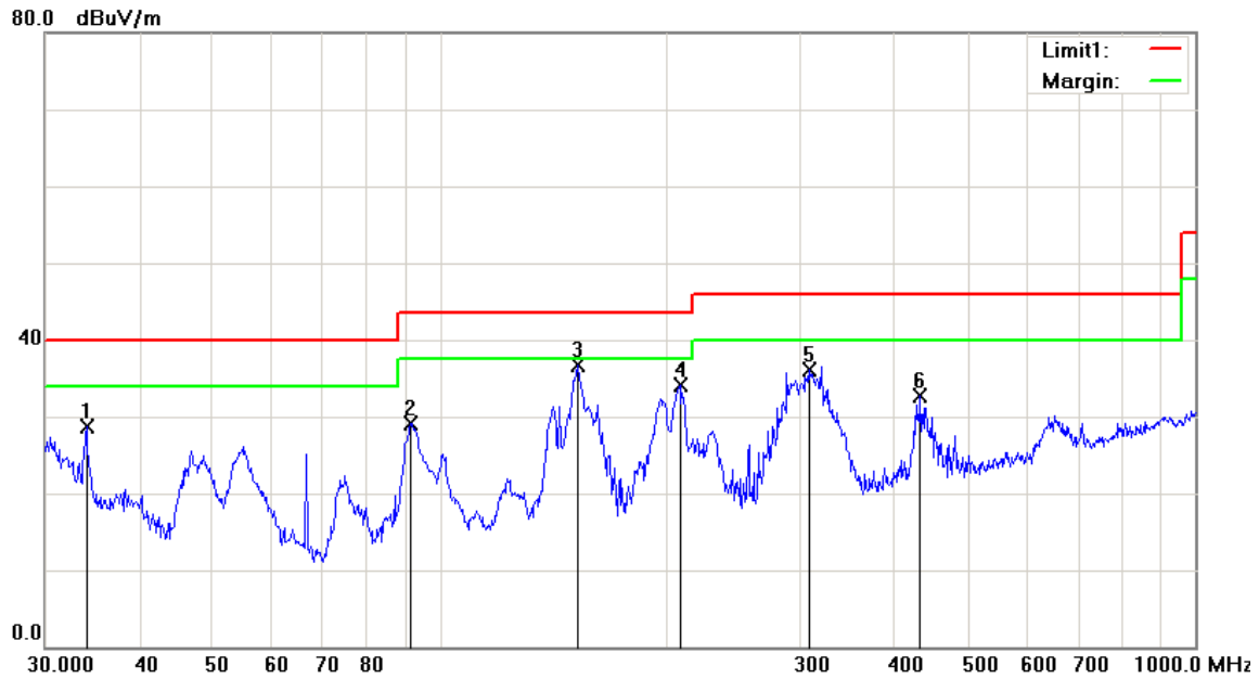
Horizontal Polarity Plot @3m
