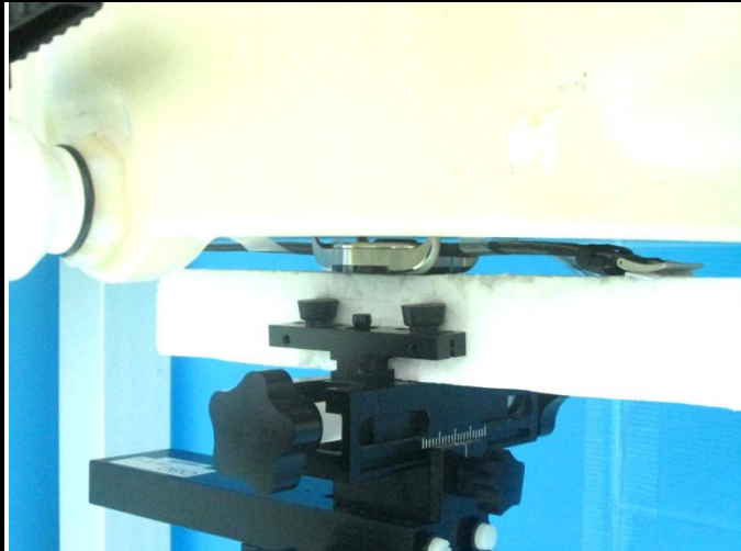
Rear Face of EUT with 0 cm Gap for Sample 4
