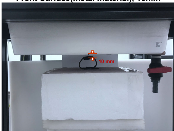
Photograph 7. Body, Front Surface(KY material), 10mm
