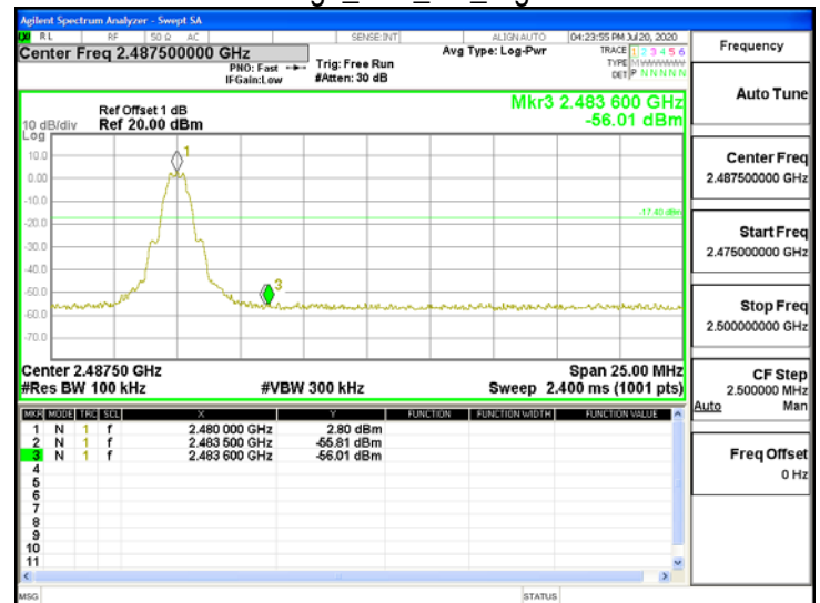
BLE\Band Edge_BLE_1M_HighCH39-2480
