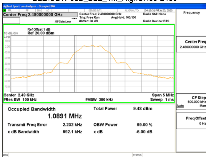
BLE\OBW 6dB_BLE_1M_HighCH39-2480
