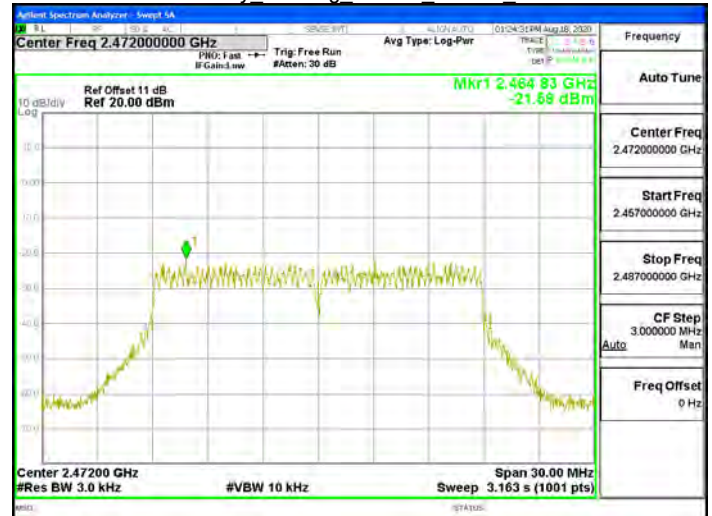
Power Density_802.11g_20MHz_Chain0_2472MHz
