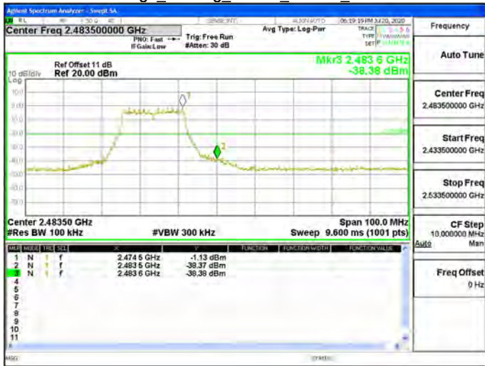
Band Edge_802.11g_20MHz_Chain0_2472MHz
