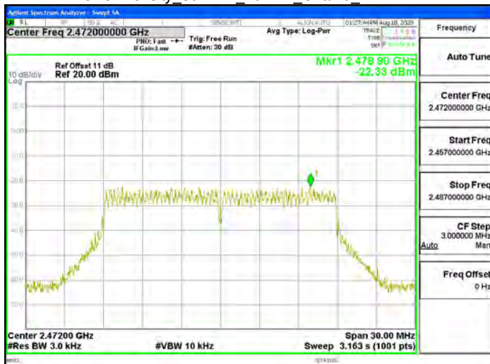
Power Density_802.11n_20MHz_Chain0_2472MHz
