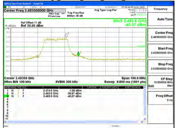
Band Edge_802.11n_20MHz_Chain0_2472MHz
