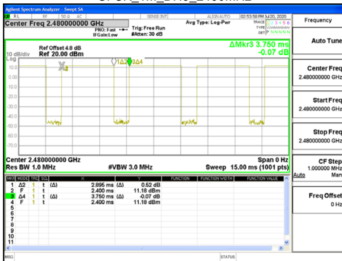
GFSK_1M_DH5_2480MHz
