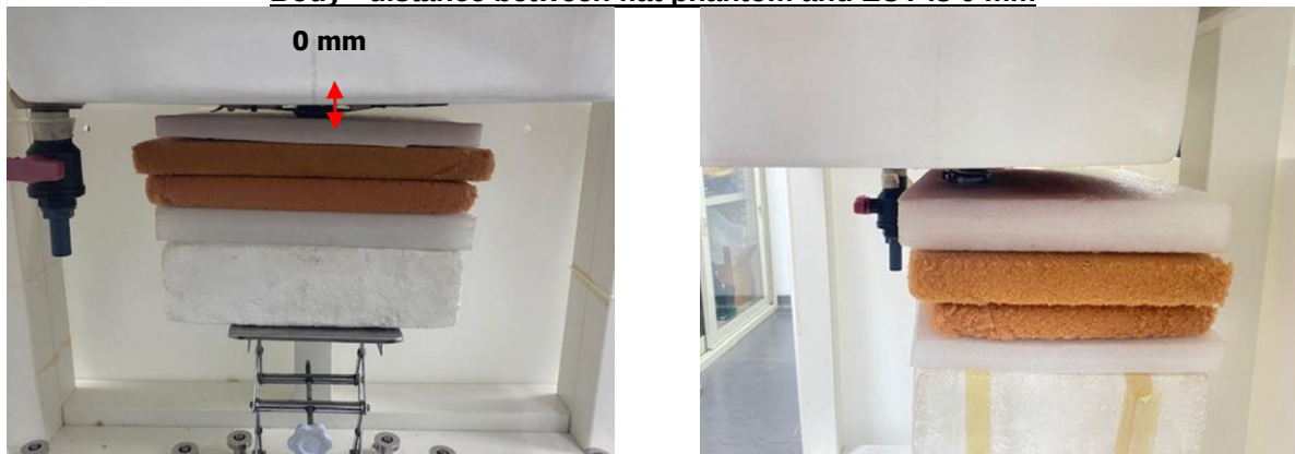
Fig.3 Back side of EUT to flat phantom
