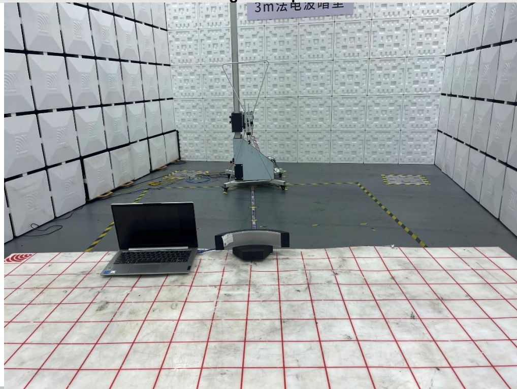
Radiated Band edge and Spurious Emission
