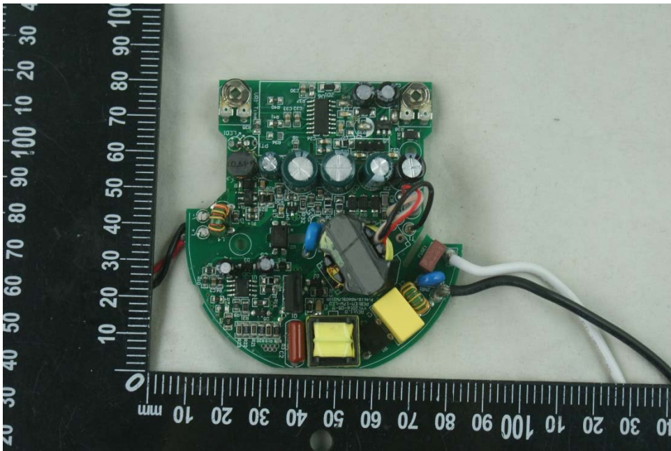
MAIN BOARD 1 FRONT VIEW
