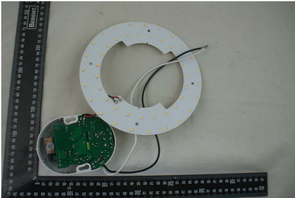
EUT UNCOVER VIEW 3
