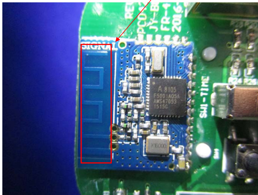
EUT- BT Module & Antenna View
