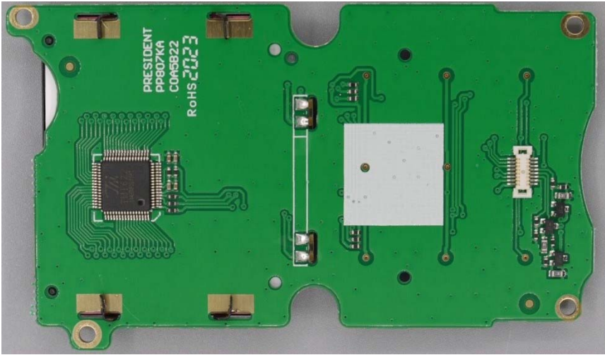
Figure E18.9 – Internal Photo – Battery Controller PCB
