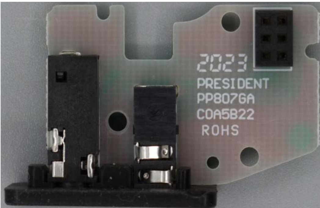
Figure E18.8 – Internal Photo – Accessory PCB Top
