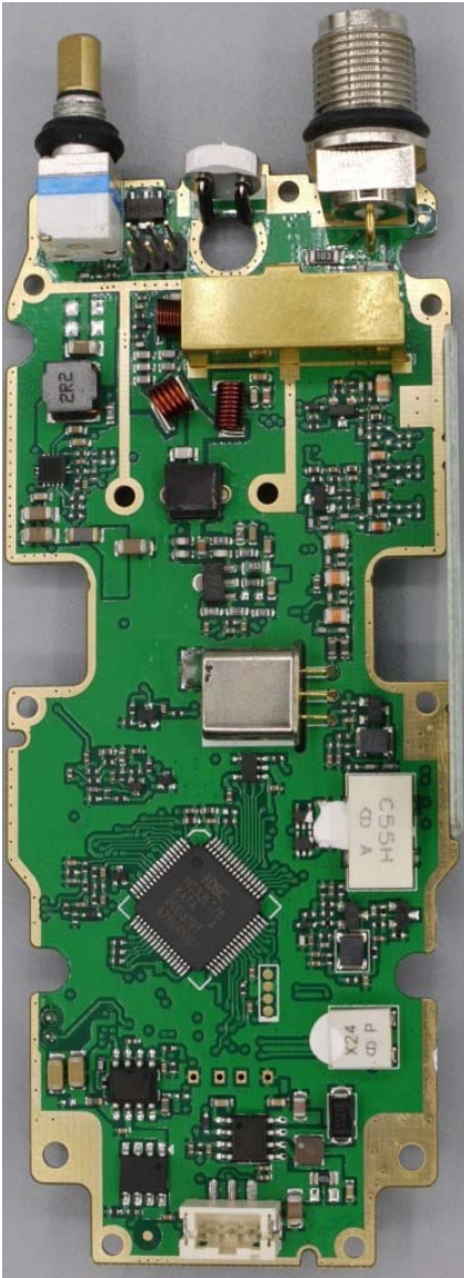
Figure E18.3 – Internal Photo – Main PCB Top
