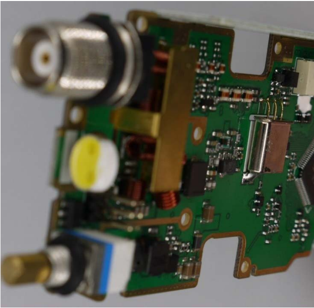
Figure E18.5 – Internal Photo – Main PCB Top End
