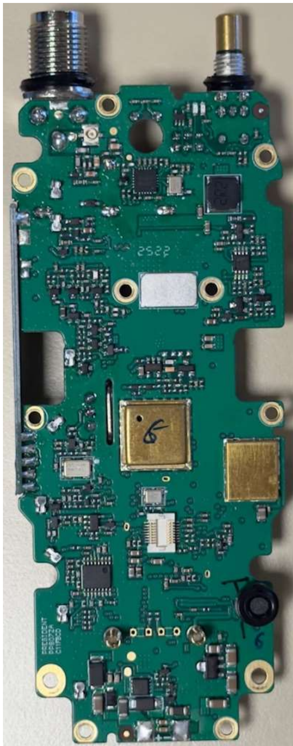
Figure E10.5 – Internal, Main PCB, Bottom
