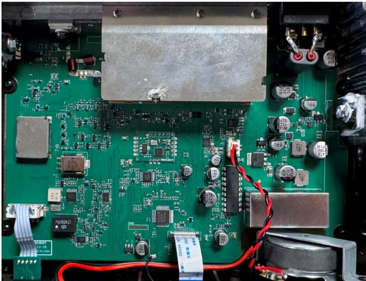
Figure E17.1 – Internal, Main PCB w/ Shields
