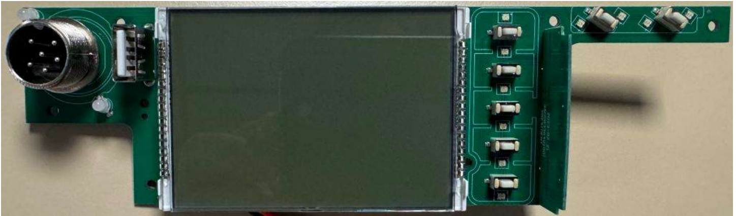
Figure E17.3 – Internal, Display PCB Front
