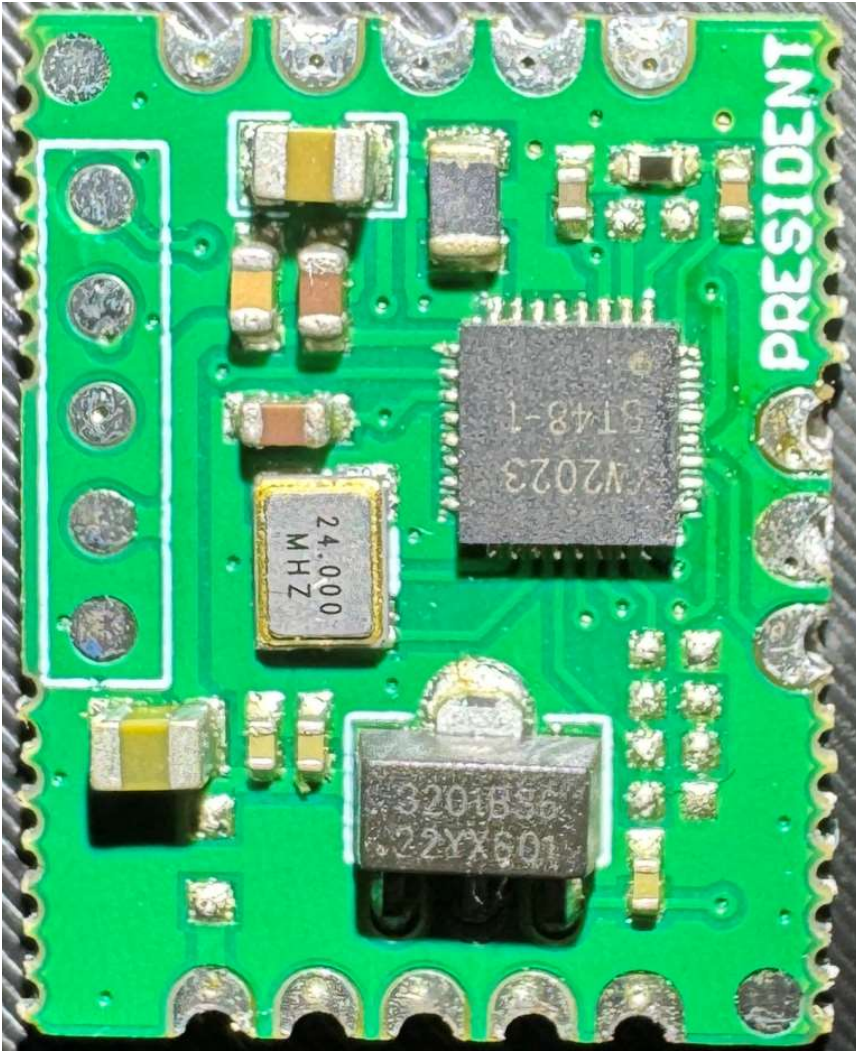
Figure E17.5 – Internal, Back Daughter PCB Top
