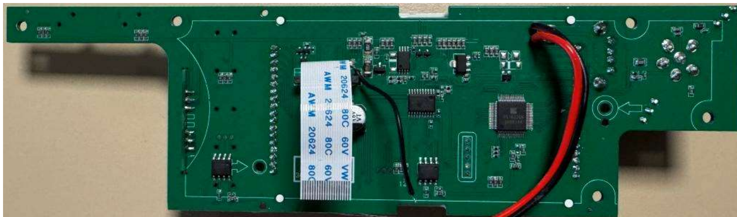
Figure E17.4 – Internal, Back Display PCB Back
