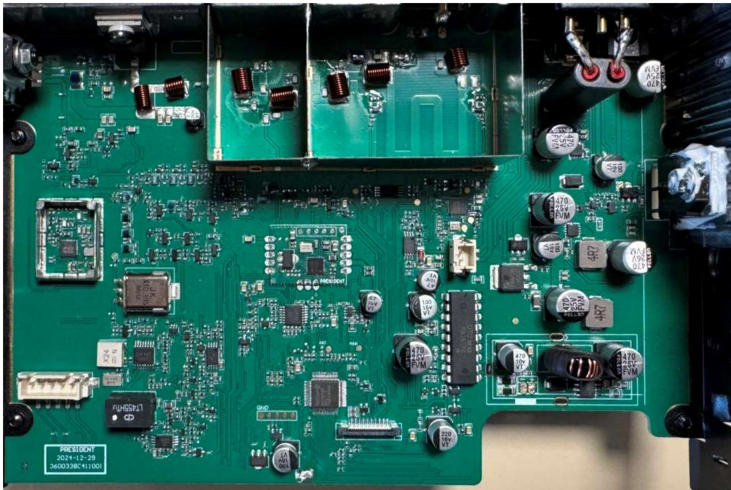
Figure E17.2 – Internal, Main w/o Shields
