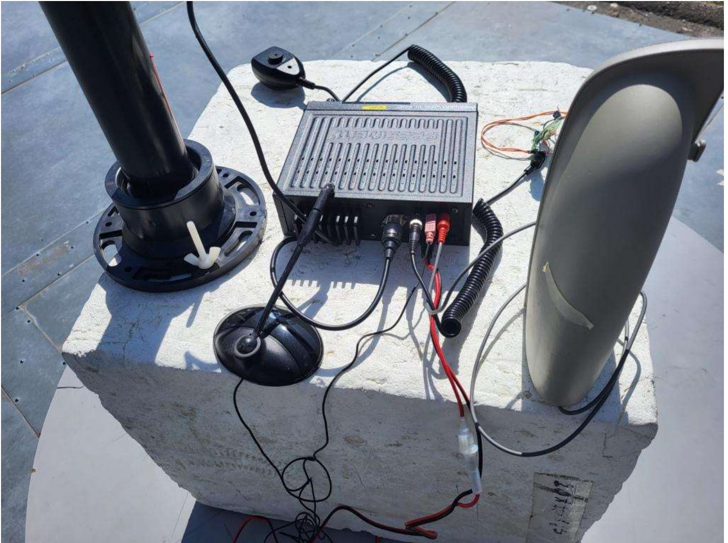
Figure E18.5 – Setup, Radiated Emissions, Accessories
