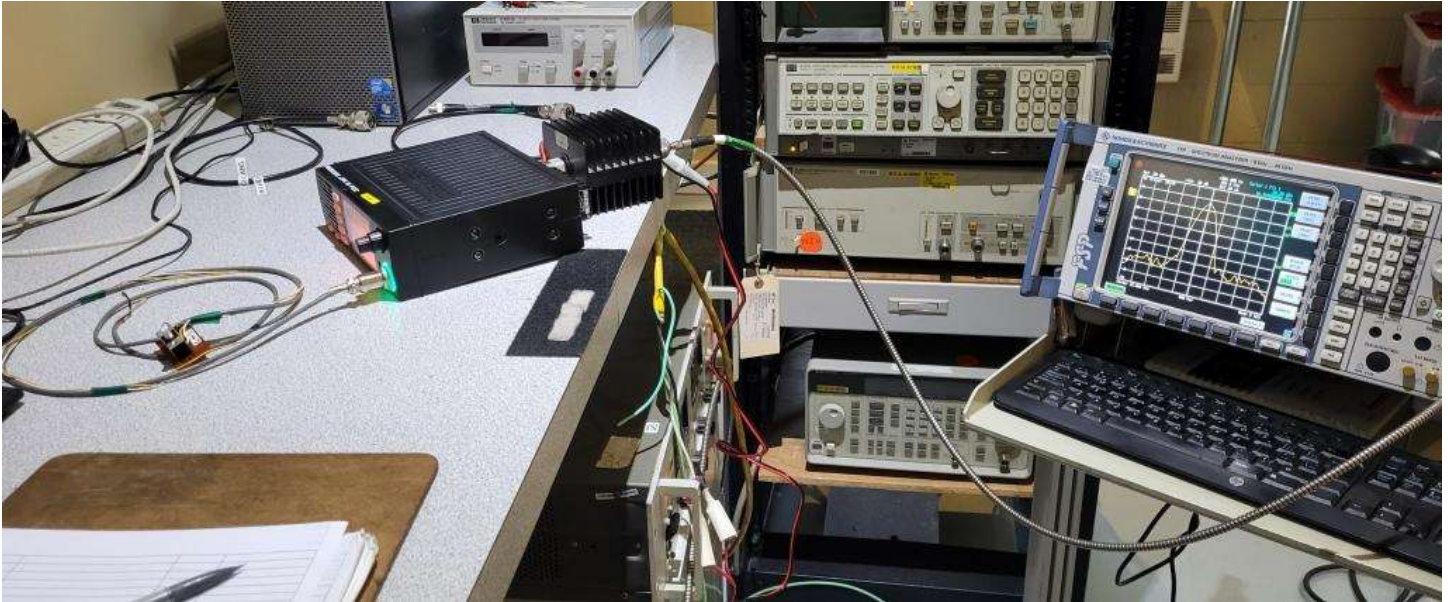
Figure E18.1 – Setup, Antenna Port Conducted
