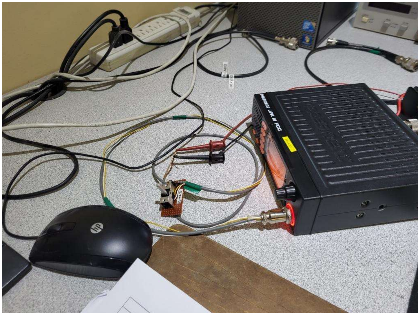
Figure E18.3 – Setup, Modulation Characteristics
