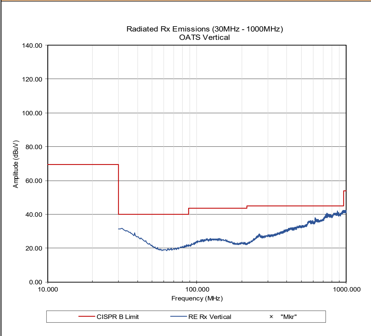
Plot 13.4– Radiated Spurious Emissions OATS, 30 - 1000MHz, Vertical
