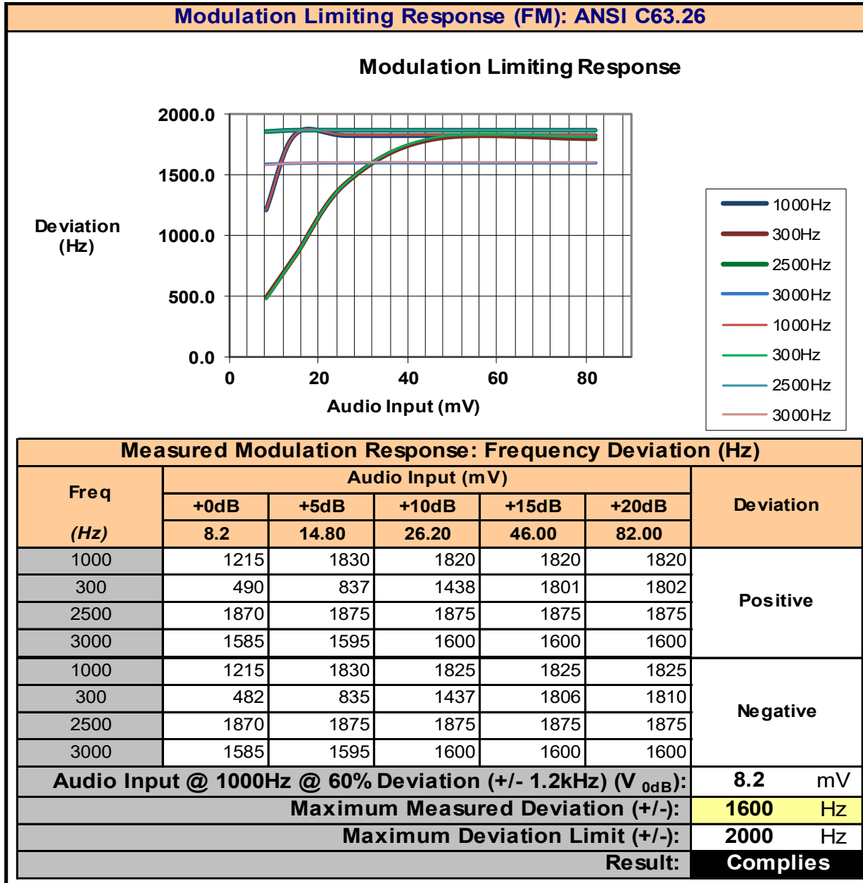
Plot 8.5 – Modulation Limiting Response, FM (ANSI C63.26)
