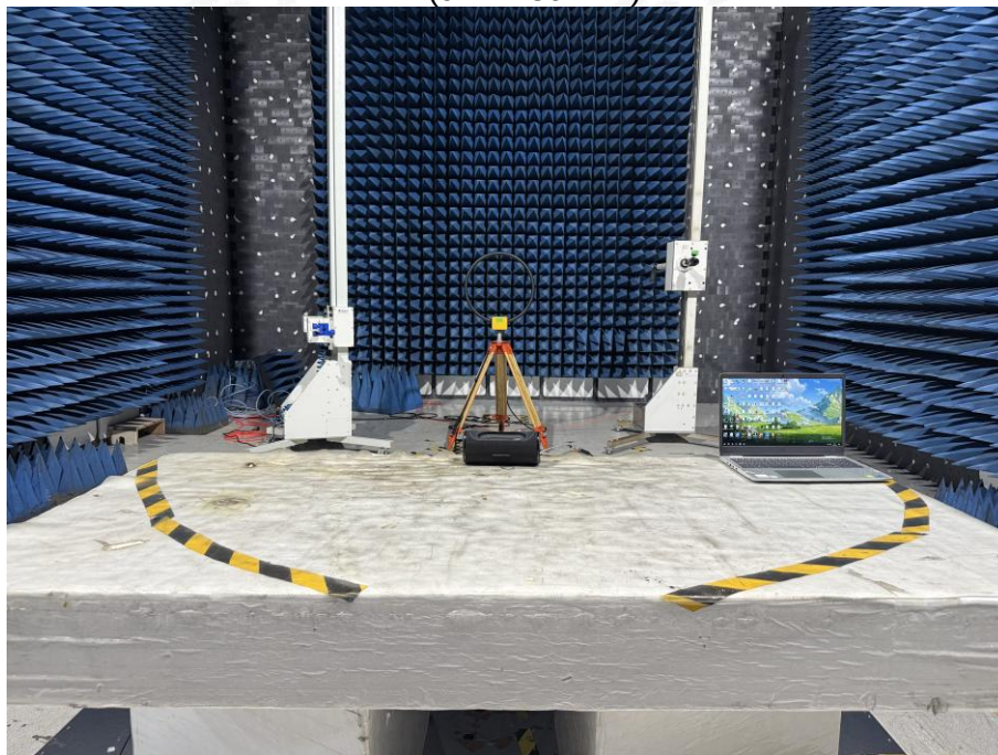
RE (9KHz-30MHz)
