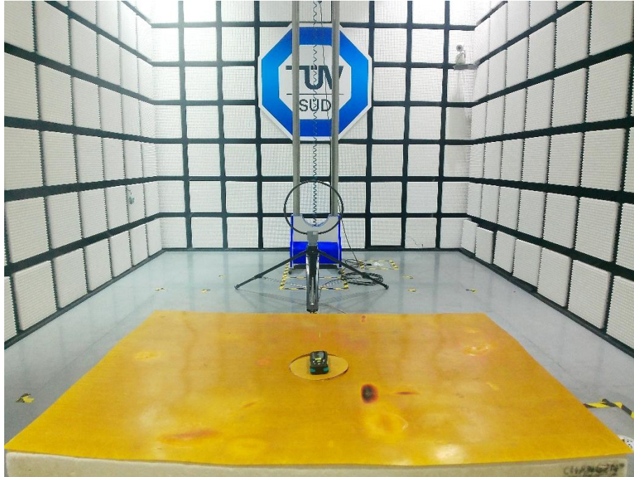
9kHz-30MHz RSE Setup
