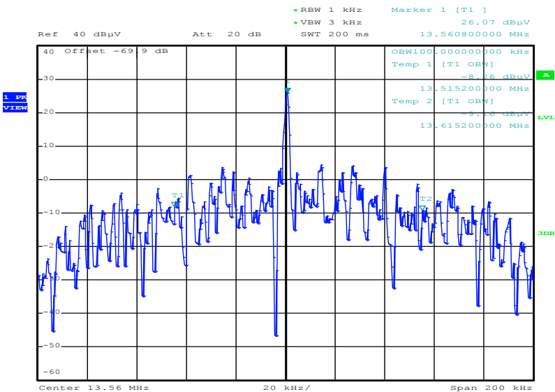
Plot 1: 99 % emission bandwidth
