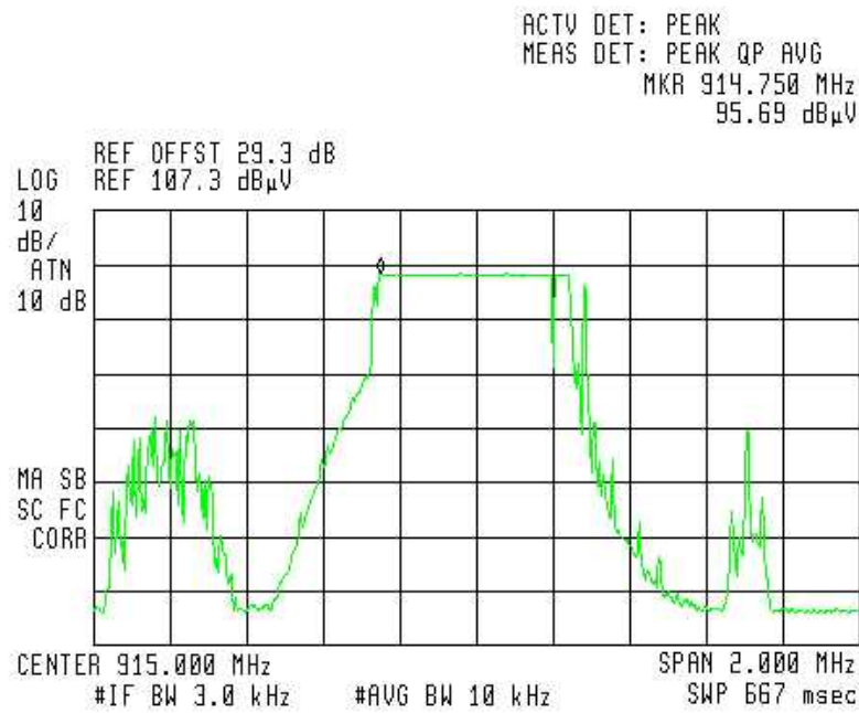
Figure 30 — 915MHz
