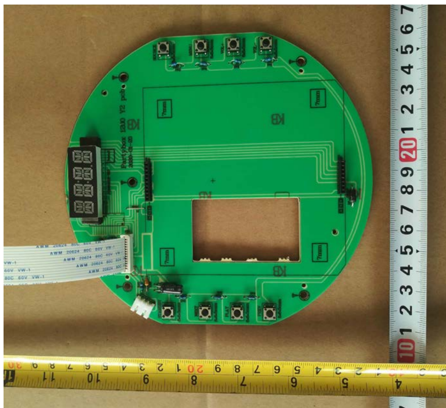
Solder Board-Component View 15
