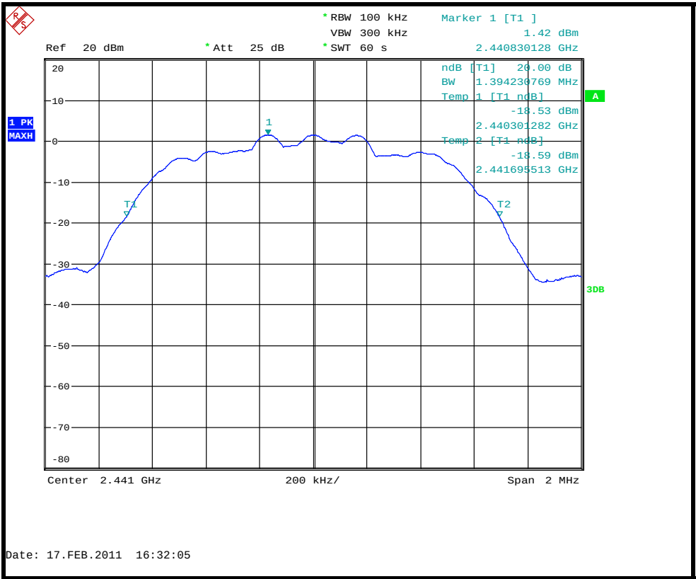
20dB Bandwidth – 3Mbps
