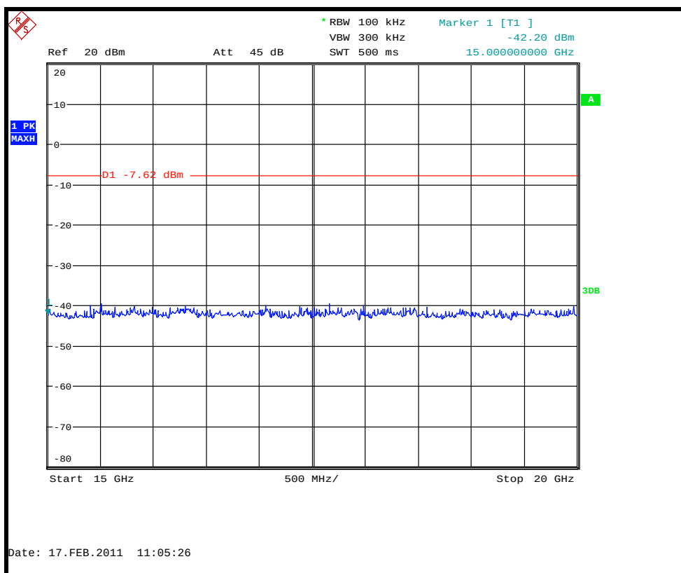
Conducted spurious emissions 15 GHz to 20 GHz – 2402.0MHz – 1Mbps
