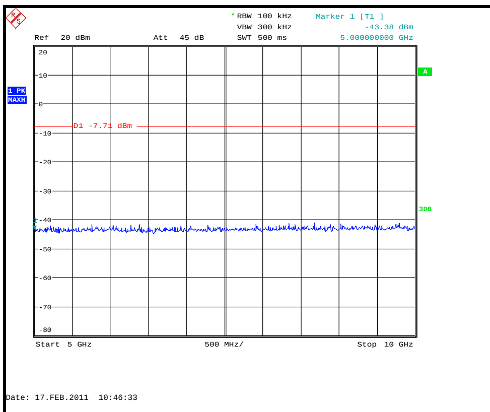
Conducted Spurious emissions 5 GHz to 10 GHz – 2441.0 MHz – 1Mbps
