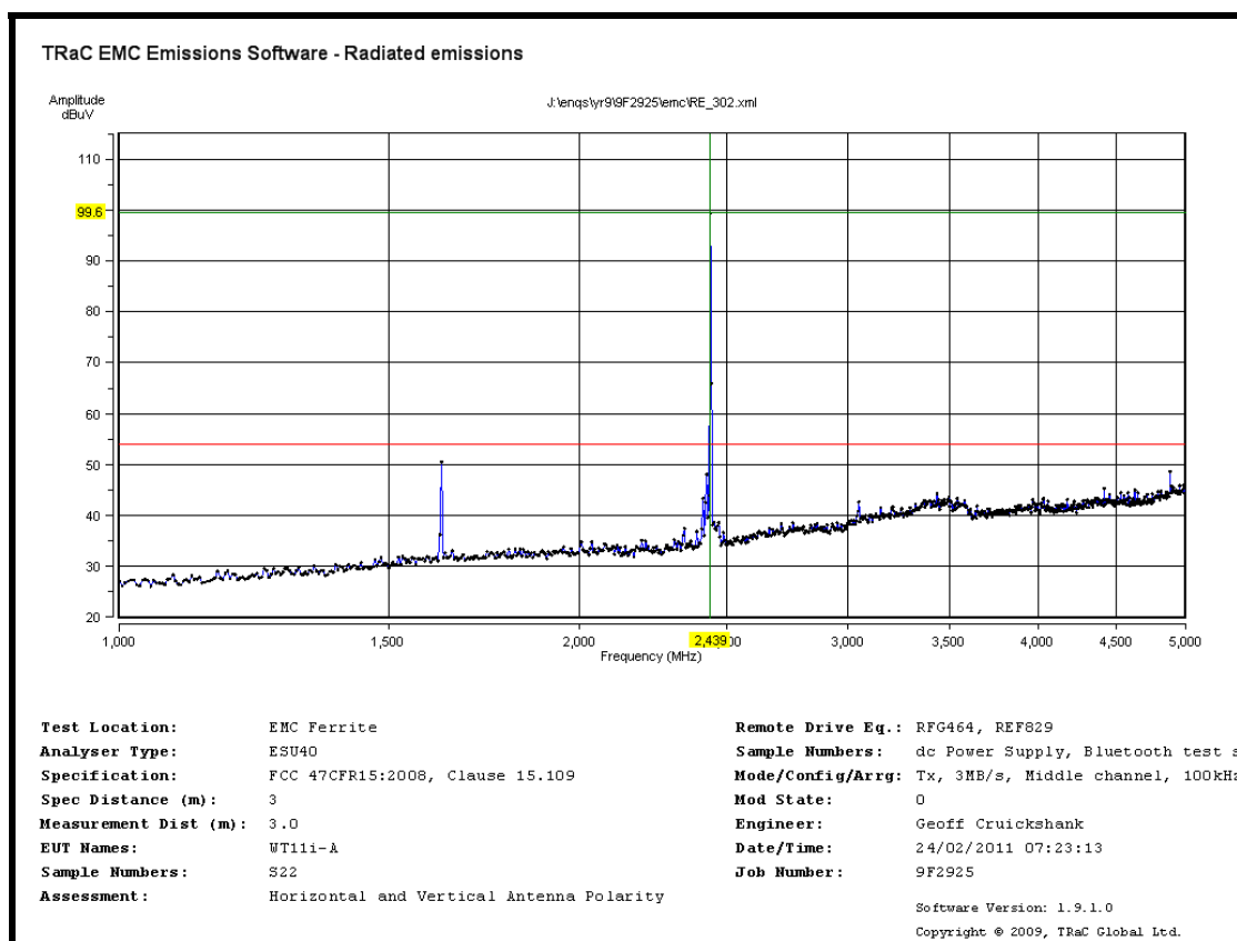
Radiated Spurious emissions 1 GHz to 5 GHz – 2441MHz – 3Mbps
