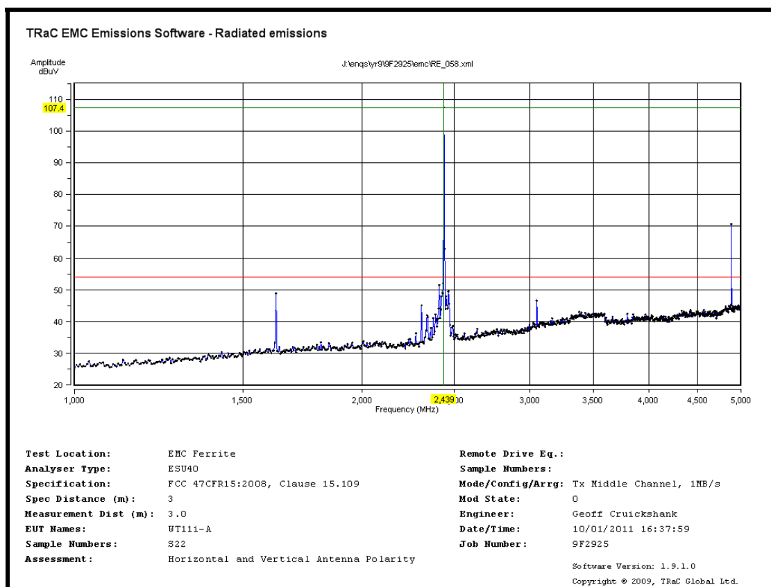
Radiated Spurious emissions 1 GHz to 5 GHz – 2441MHz – 1Mbps
