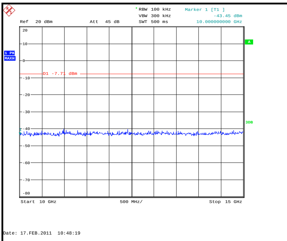
Conducted Spurious emissions 10 GHz to 15GHz – 2441.0 MHz – 1Mbps
