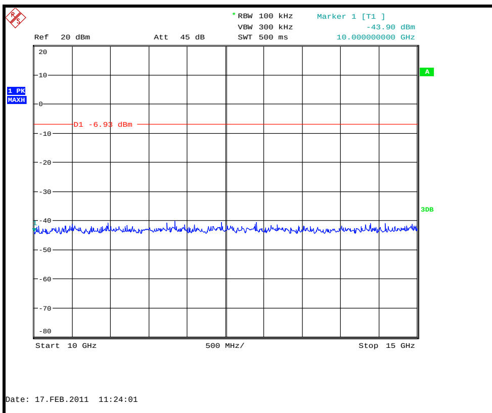
Conducted Spurious emissions 10 GHz to 15 GHz– 2480.0MHz – 1Mbps
