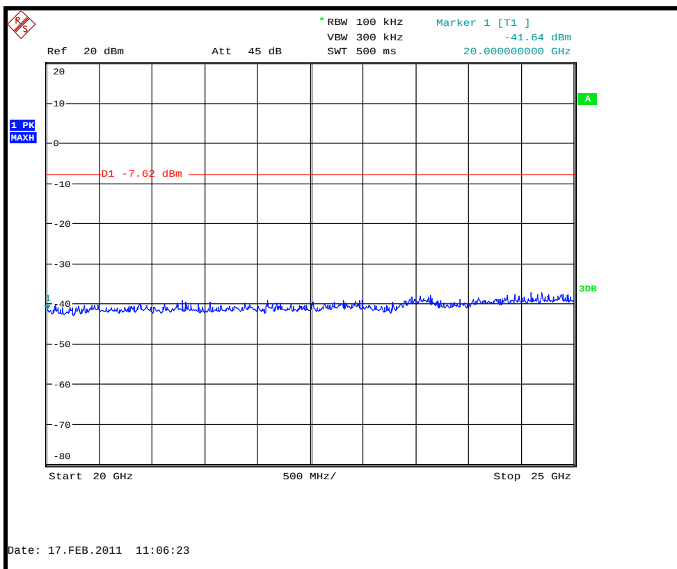
Conducted spurious emissions 20 GHz to 25 GHz – 2402.0MHz 1Mbps
