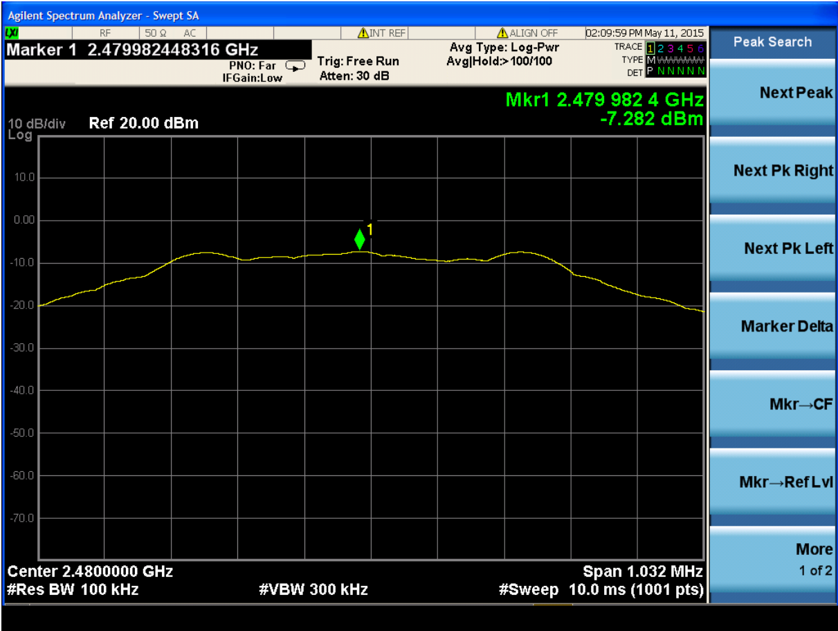
(Plot 4.4.1 C: Channel 39: 2480 MHz @ GFSK
