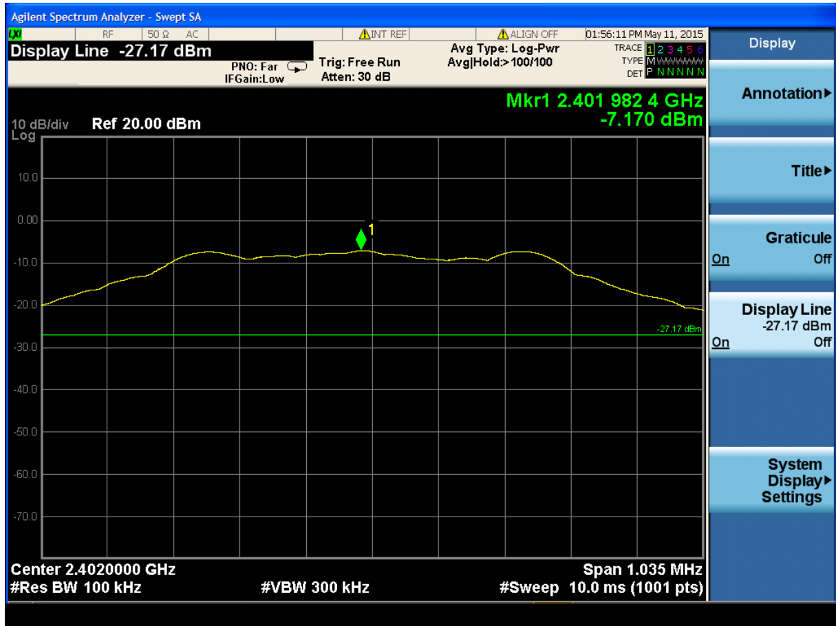
(Plot 4.6.1 A1: Channel 00: 2402MHz @ GFSK)
