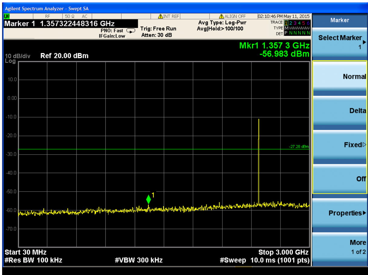
(Plot 4.6.1 C2: Channel 39: 2480MHz @ GFSK)
