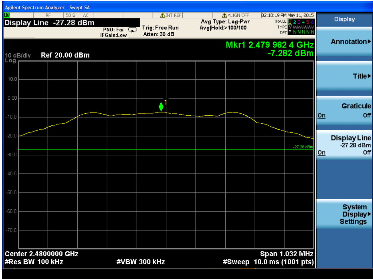
(Plot 4.6.1 C1: Channel 39: 2480MHz @ GFSK)
