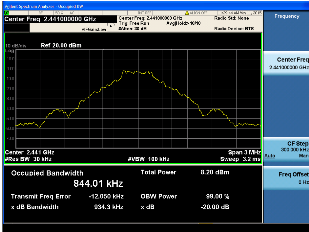
(Plot 4.4.1 B: Channel 39: 2441MHz @ GFSK)
