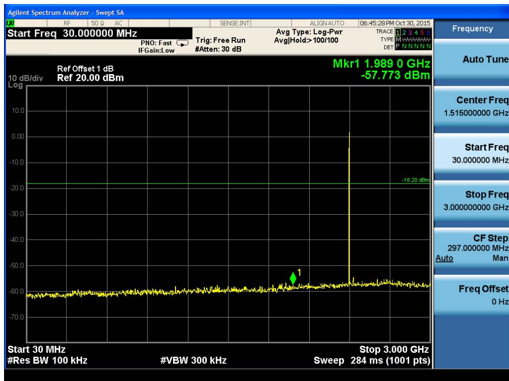
(Plot 4.9.2 A2: Channel 0: 2402MHz @ @ 8DPSK)
