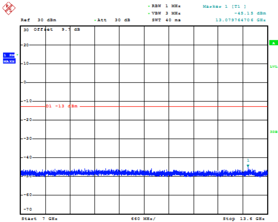
(Plot 4.5.1 A4: Channel 9262: 1852.4MHz @ Traffic WCDMA Band II)
