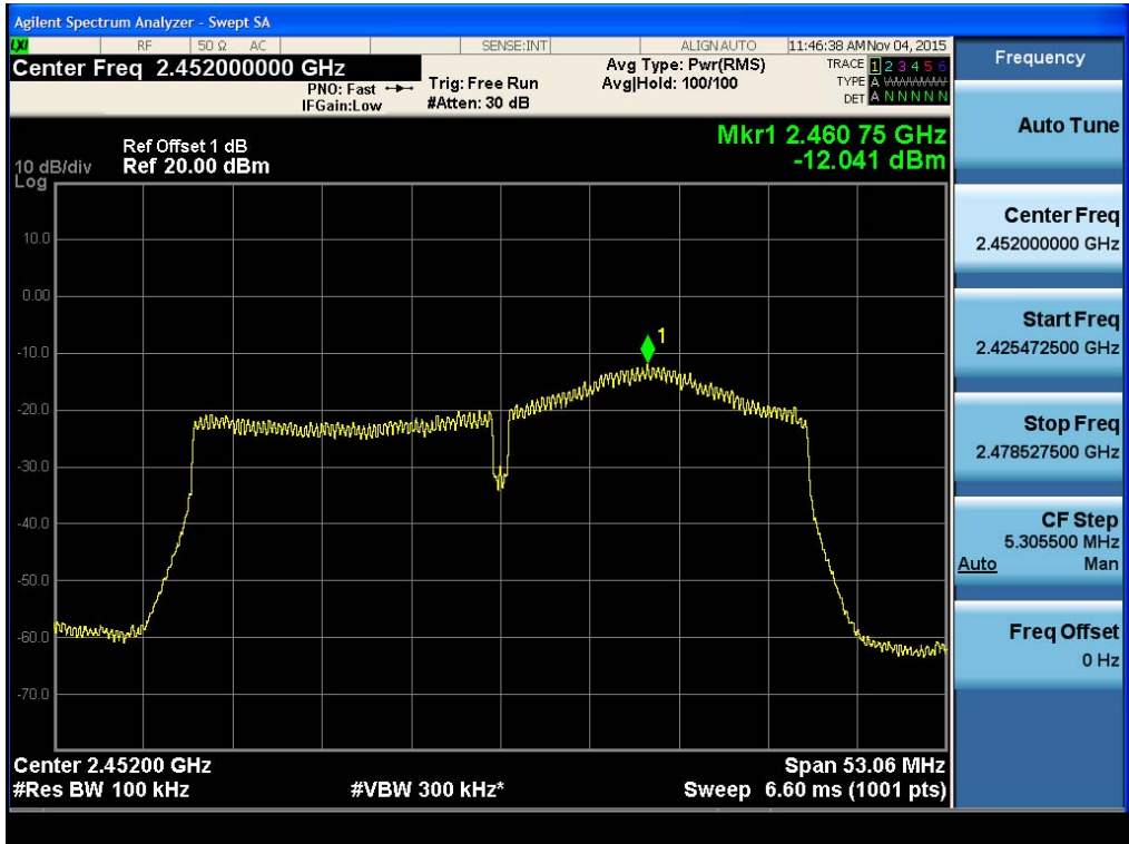
(Plot 4.4.4 C: Channel 9: 2452MHz @ 802.11n HT40)
