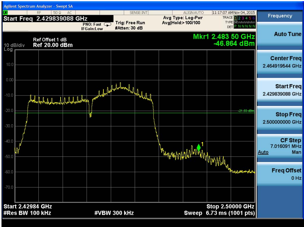
(Plot 4.5.2.4 B: Channel 9: 2452MHz @ 802.11n HT40)
