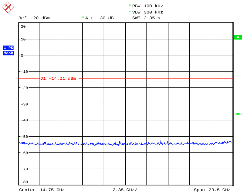
(Plot 4.6.1 B2: Channel 6: 2437MHz @ 802.11b)
