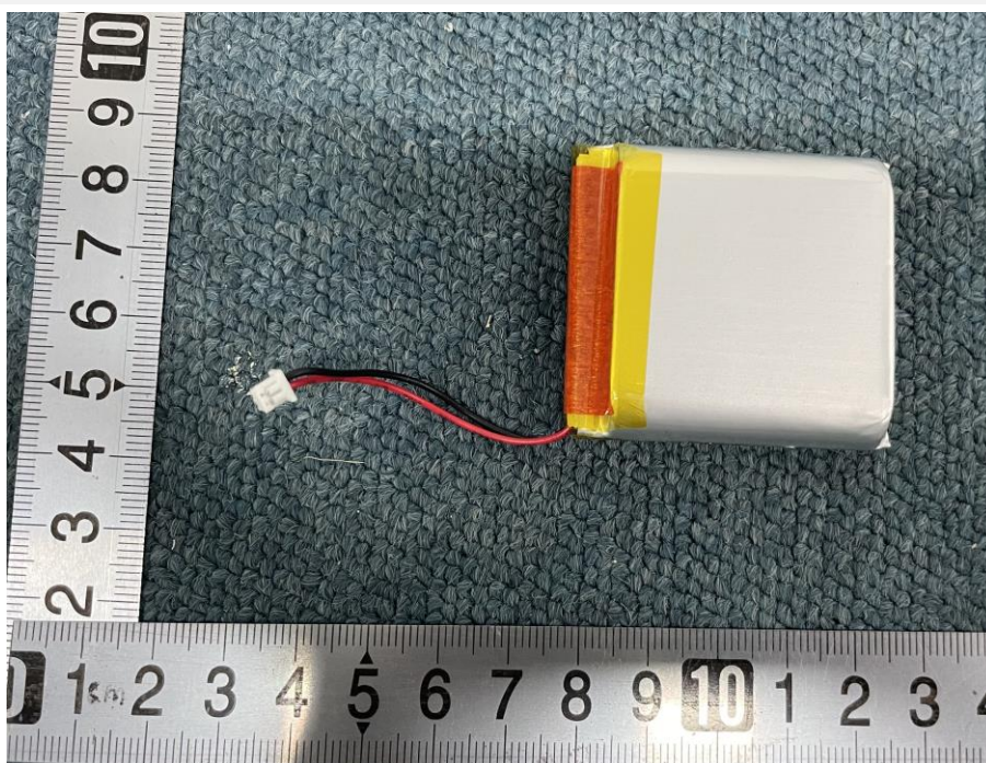
BATTERY (FRONT)
