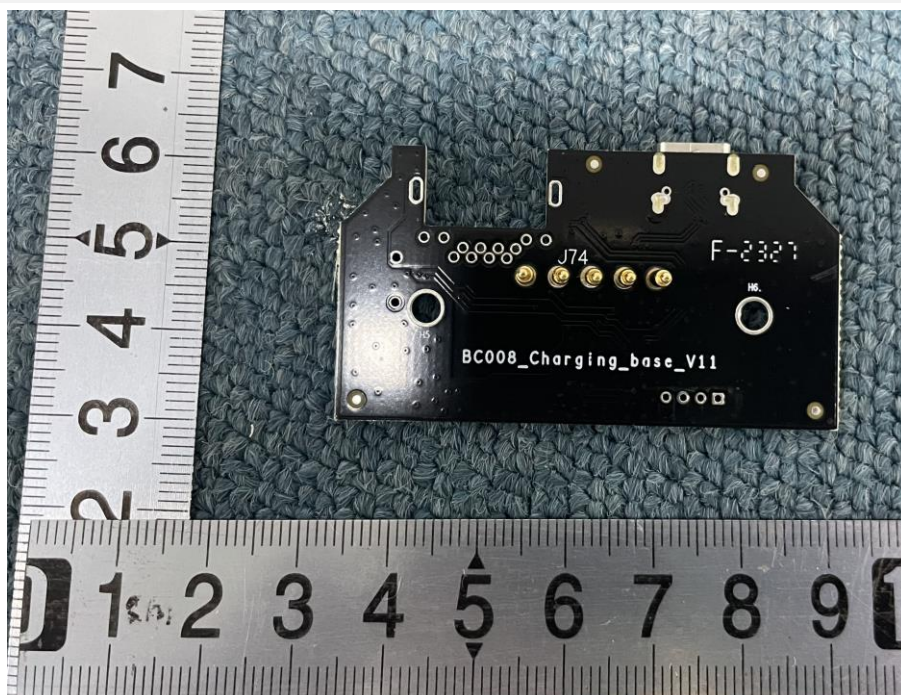
SECONDARY BOARD 2 REAR VIEW
