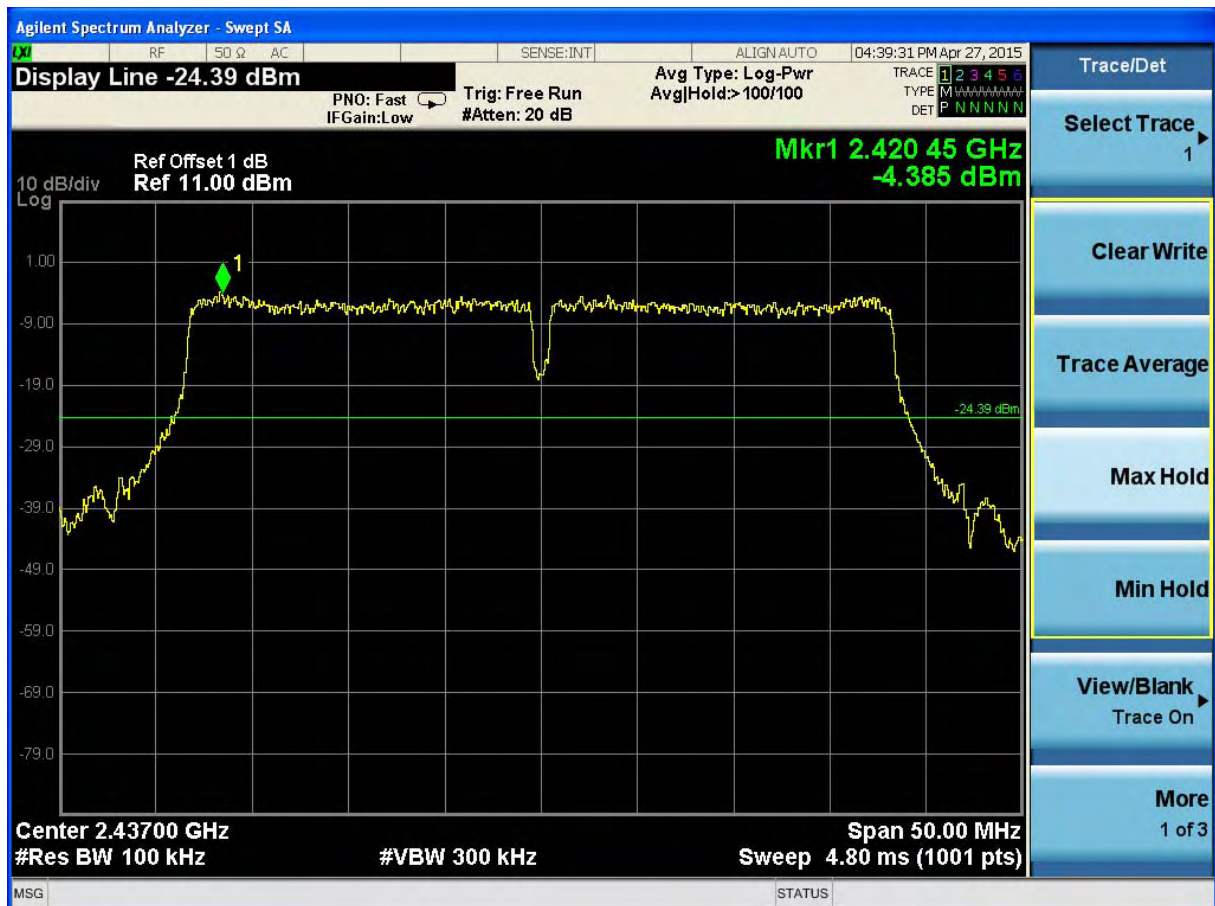
(Plot 4.7.4 B1: Channel 6: 2437MHz @ 802.11n HT40)
