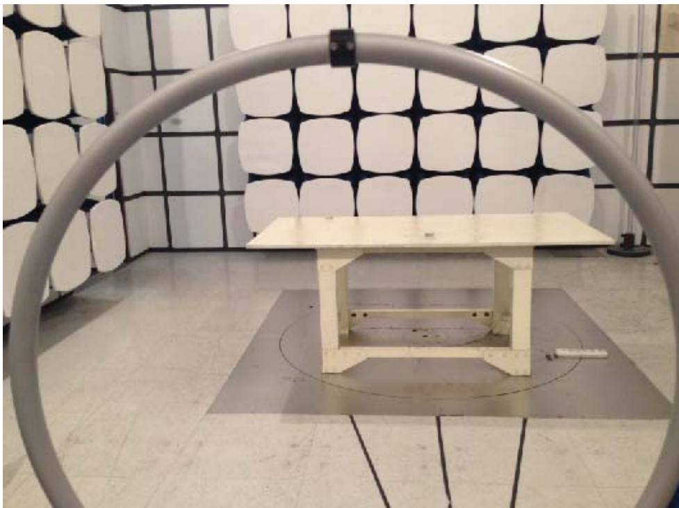
RE 9kHz-30MHz
