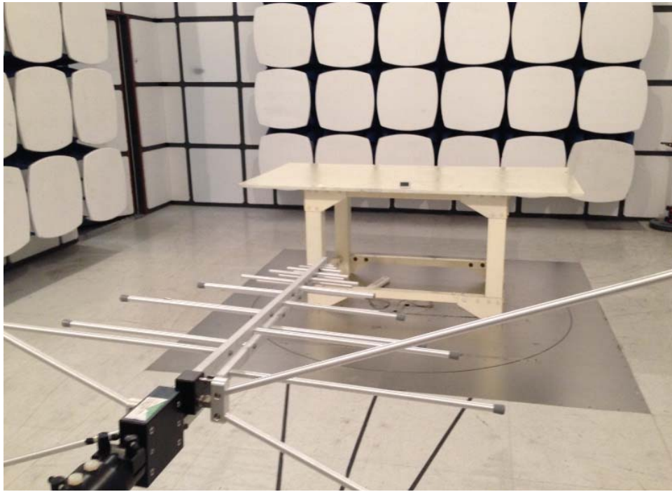
RE 30MHz-1GHz
