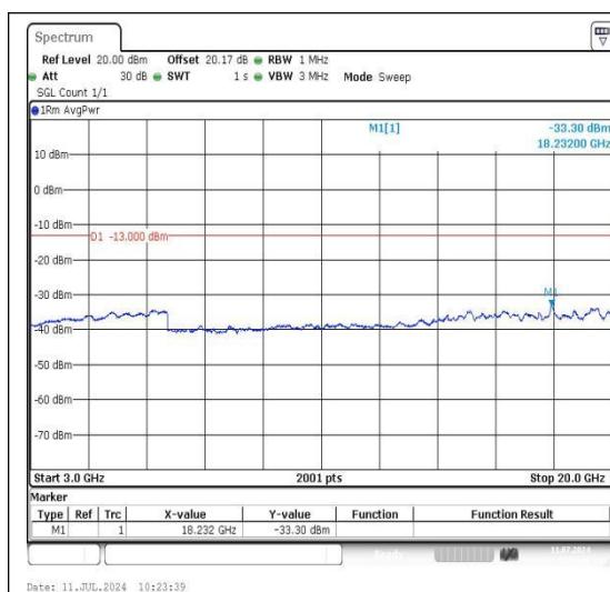
Band2_20MHz_QPSK_18700_1RB#0_3000~20000_3000~20000
