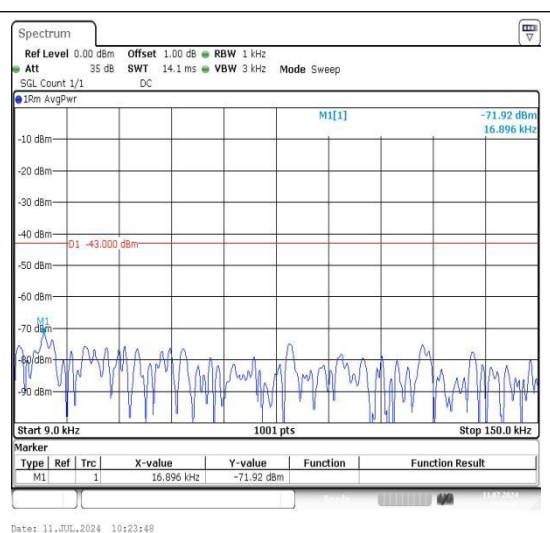
Band2_20MHz_16QAM_18700_1RB#0_0.009~0.15_0.009~0.15
