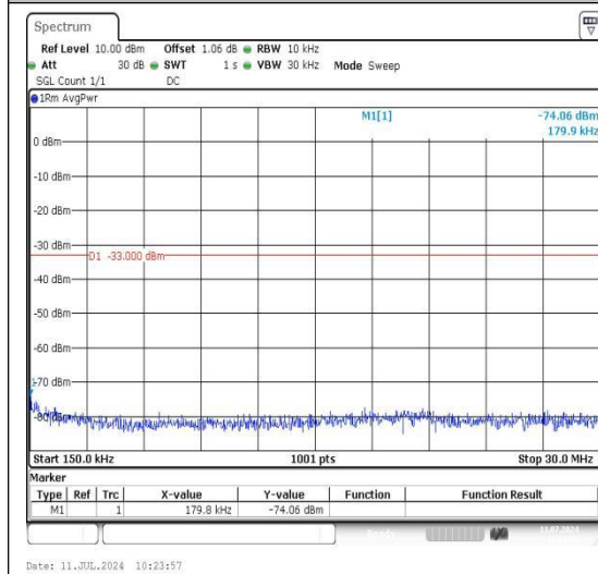
Band2_20MHz_16QAM_18700_1RB#0_0.15~30_0.15~30
