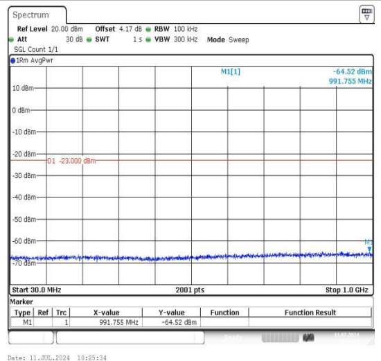
Band2_20MHz_16QAM_18900_1RB#0_30~1000_30~1000
