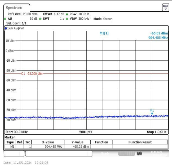
Band2_20MHz_16QAM_18700_1RB#0_30~1000_30~1000
