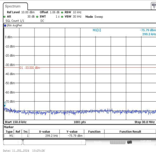
Band2_20MHz_16QAM_18900_1RB#0_0.15~30_0.15~30
