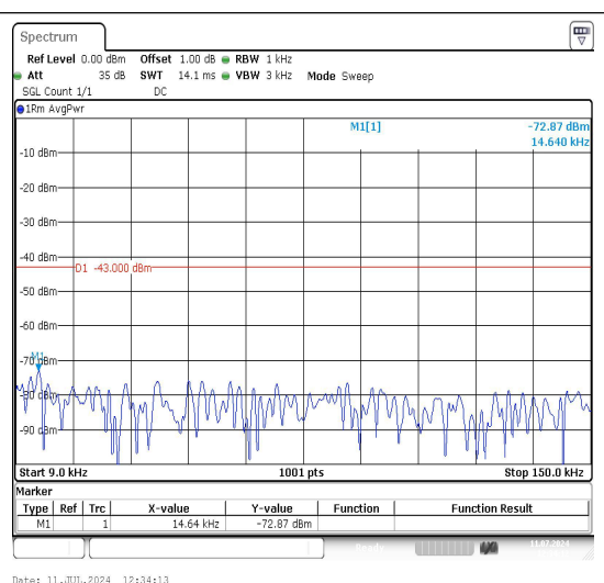
Band4_5MHz_16QAM_19975_1RB#0_0.009~0.15 _0.009~0.15
