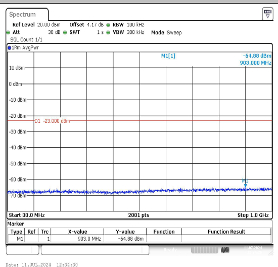
Band4_5MHz_16QAM_19975_1RB#0_30~1000_3 0~1000
