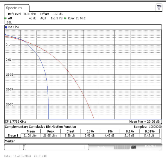
Band66-1.4MHz-16QAM-132665-1RB#0-PASS
