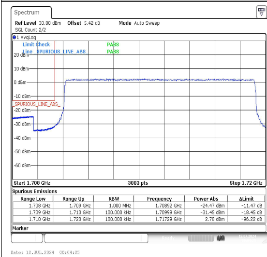
Band66_10MHz_QPSK_132022_50RB#0
