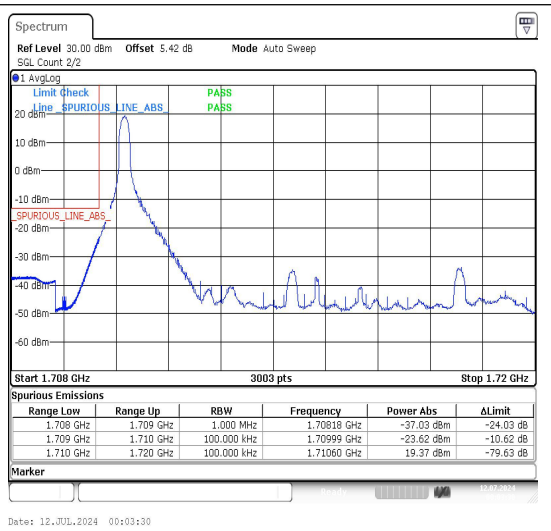
Band66_10MHz_16QAM_132022_1RB#0
