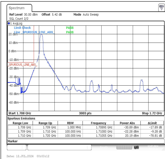
Band66_10MHz_QPSK_132022_1RB#0
