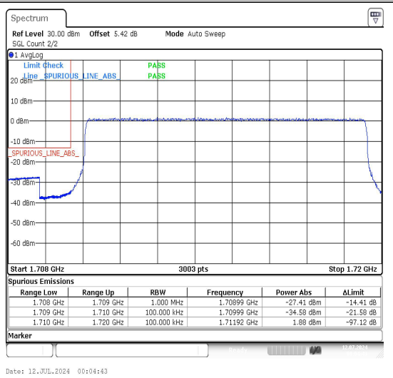
Band66_10MHz_16QAM_132022_50RB#0
