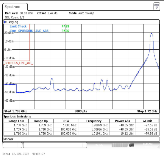
Band66_10MHz_16QAM_132022_1RB#49
