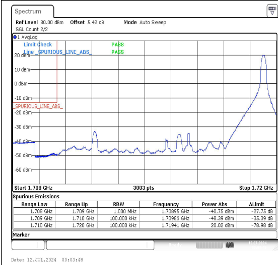
Band66_10MHz_QPSK_132022_1RB#49
