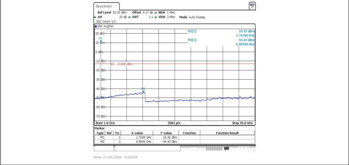
Band4-1513-2-1000~20000MHz-PASS
