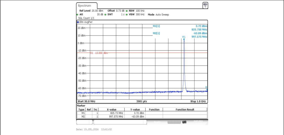
Band5-4132-2-30~1000MHz-PASS
