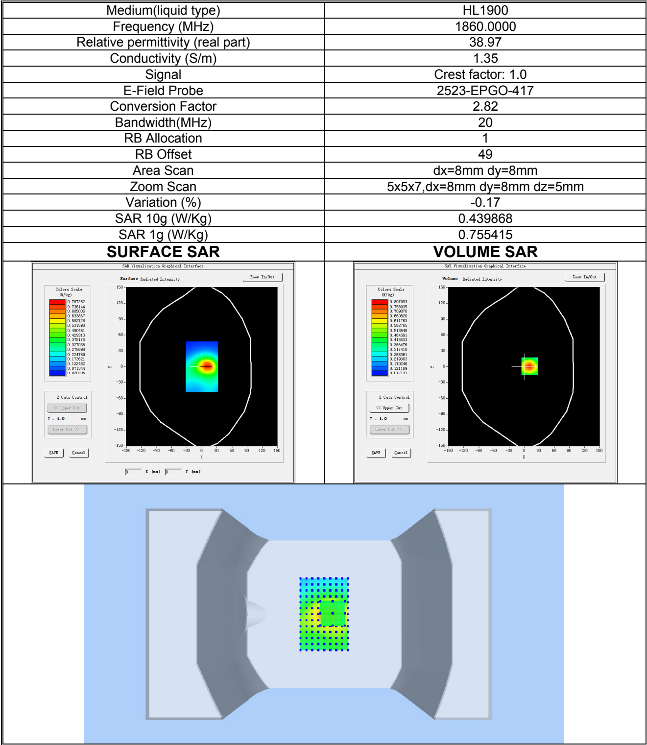
Plot 18:LTE BAND 2, Low channel (Hotspot, Back Side) Product Description:Smart Phone Test Date: 2025-12-01
