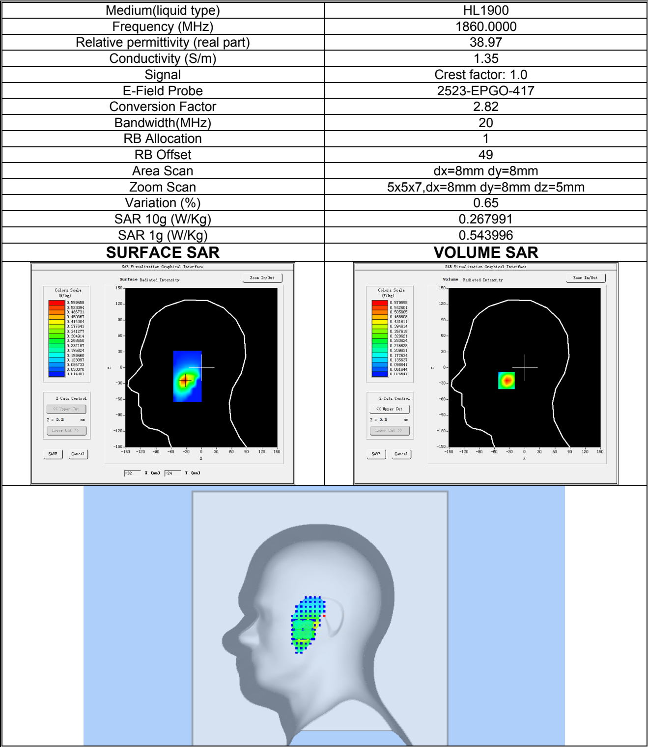
Plot 16:LTE BAND 2, Low channel (Right Head Cheek) Product Description:Smart Phone Test Date: 2025-12-01
