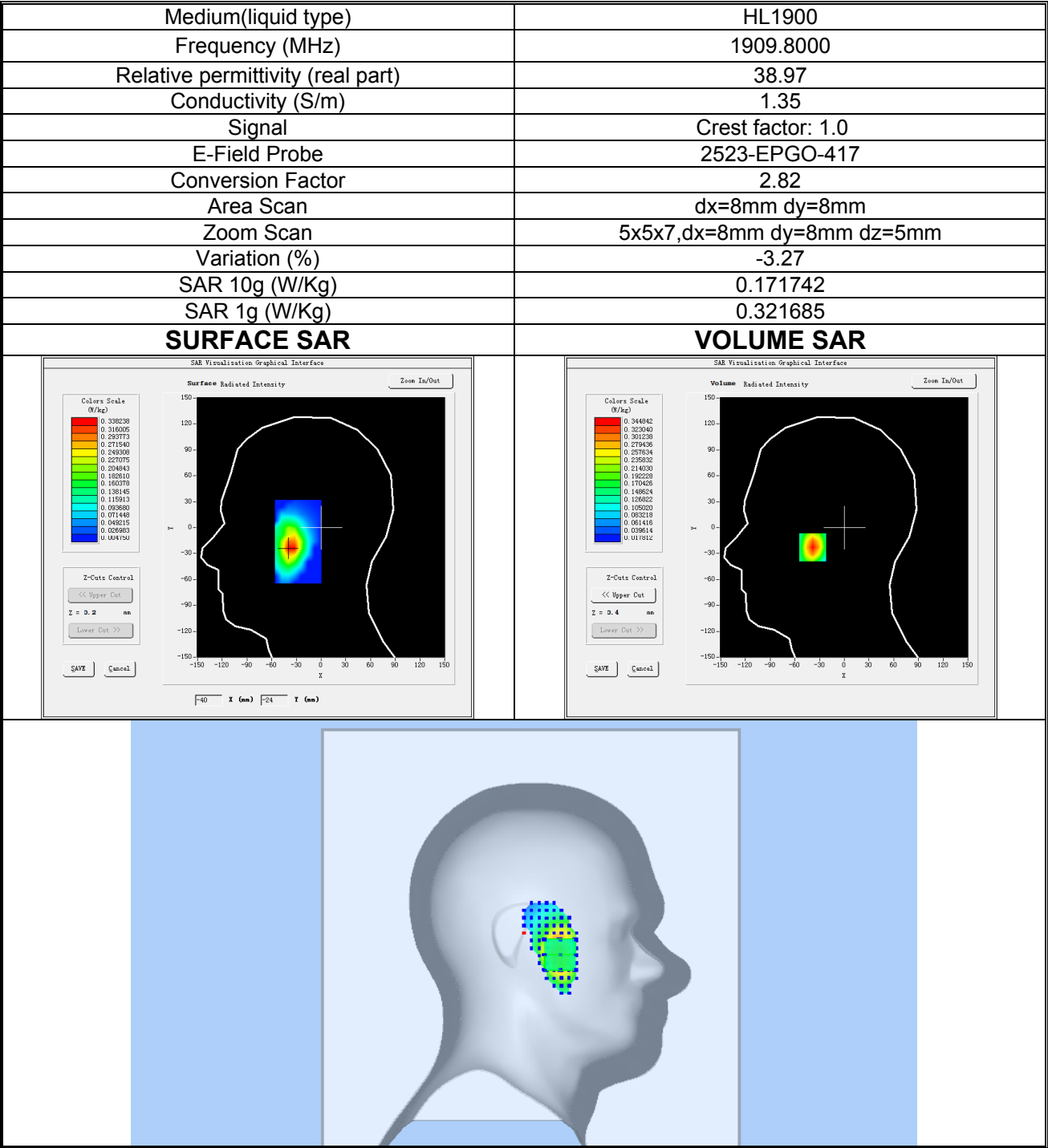
Plot 4: GSM 1900, High channel (Left Head Cheek) Product Description: Smart Phone Test Date: 2025-12-01
