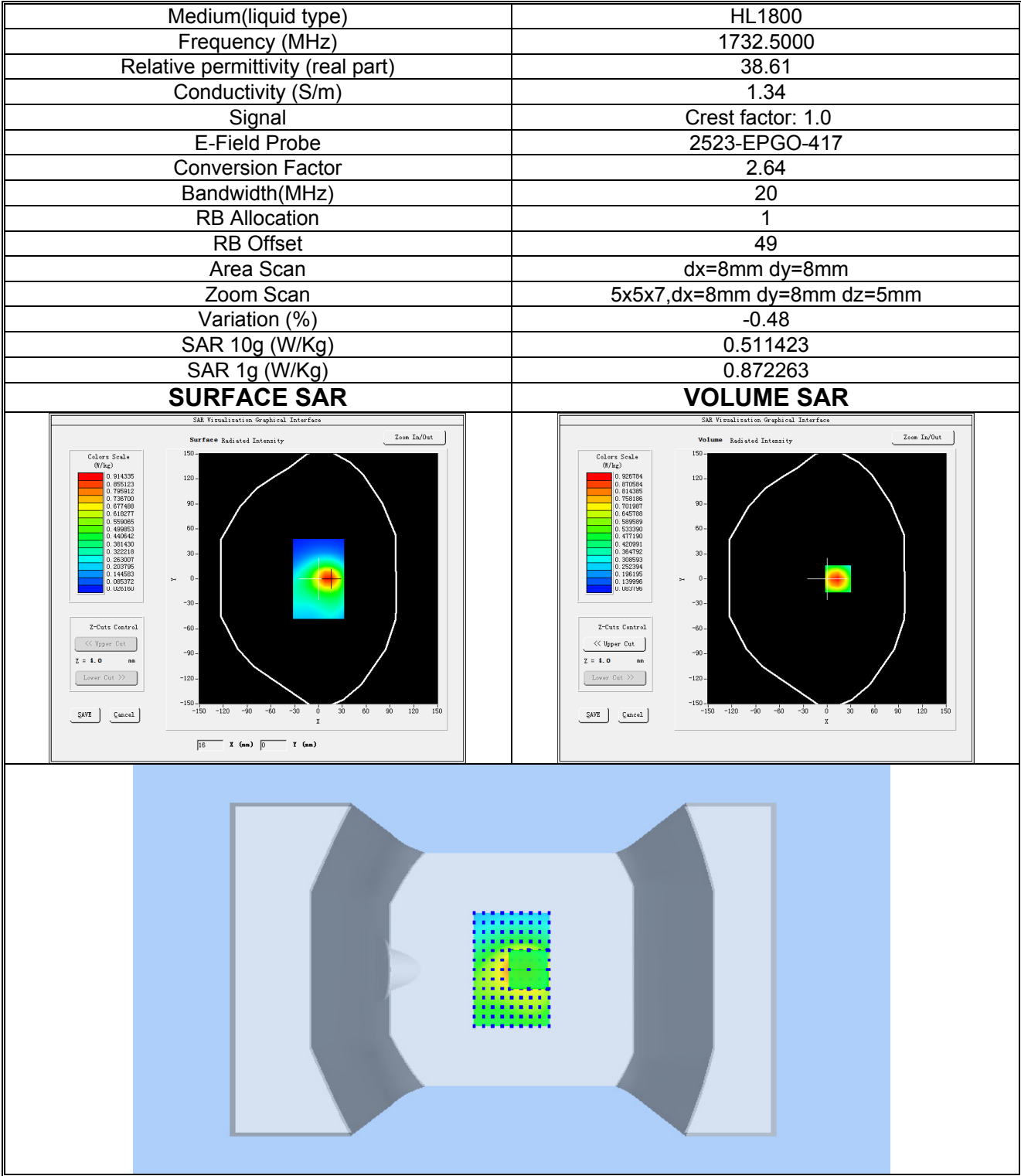
Plot 21: LTE BAND 4, Middle channel (Hotspot, Back Side) Product Description: Smart Phone Test Date: 2025-12-01
