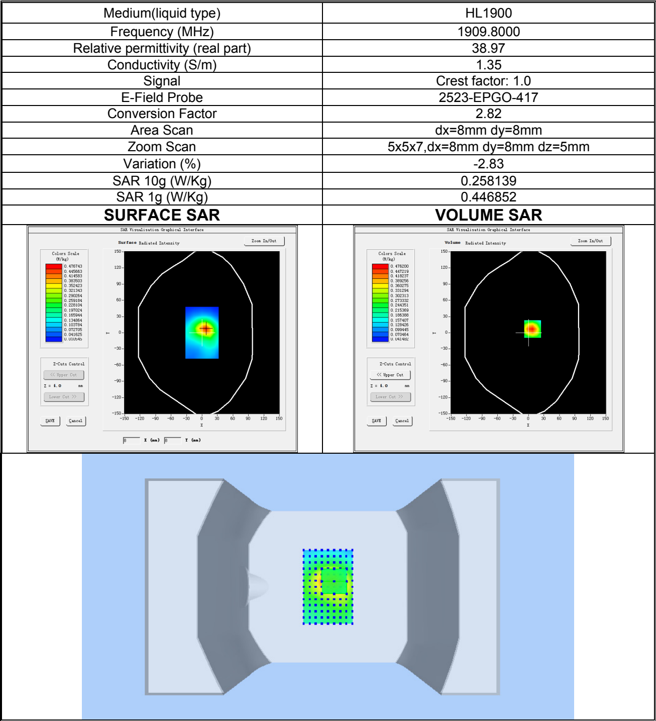
Plot 5: GSM 1900, High channel (Body-worn, Back Side) Product Description: Smart Phone Test Date: 2025-12-01
