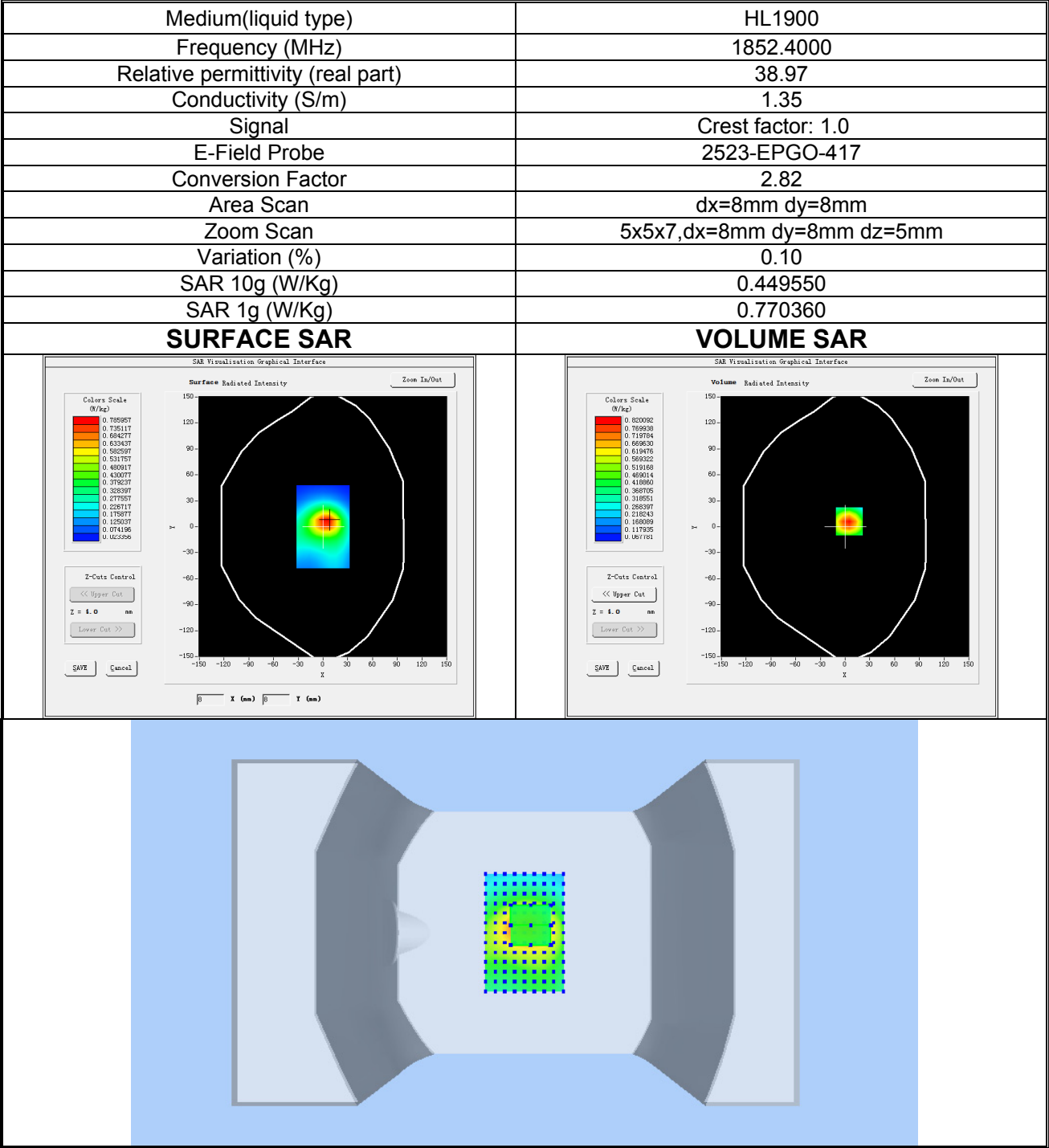
Plot 8: WCDMA BAND II, Low channel (Body-worn, Back Side) Product Description: Smart Phone Test Date: 2025-12-01
