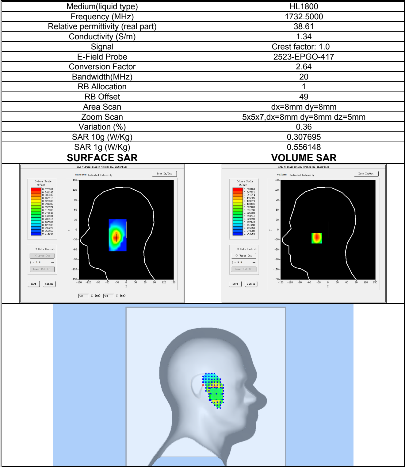
Plot 19:LTE BAND 4, Middle channel (Left Head Cheek) Product Description: Smart Phone Test Date: 2025-12-01
