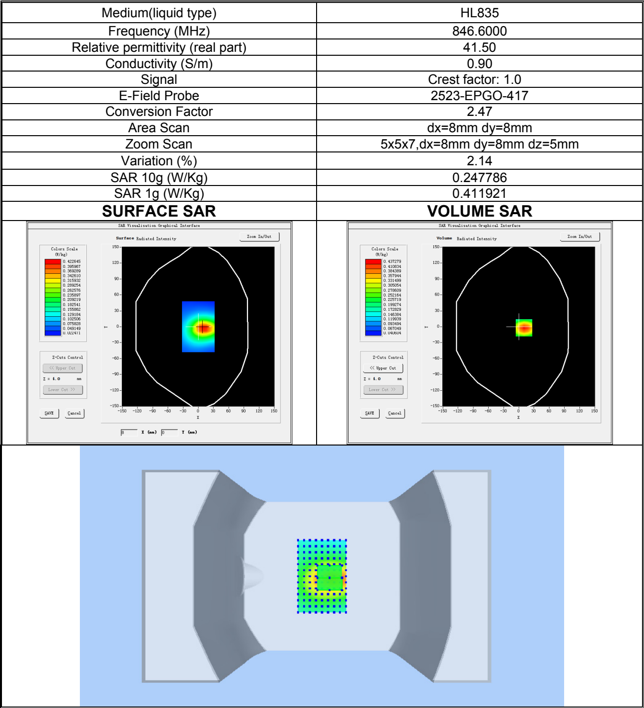
Plot 15: WCDMA BAND V, High channel (Hotspot, Back Side) Product Description: Smart Phone Test Date: 2025-12-02
