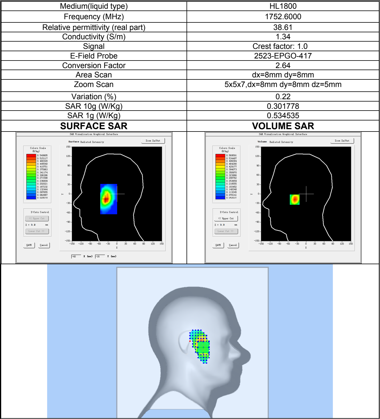
Plot 10: WCDMA BAND IV, High channel (Left Head Cheek) Product Description: Smart Phone Test Date: 2025-12-01
