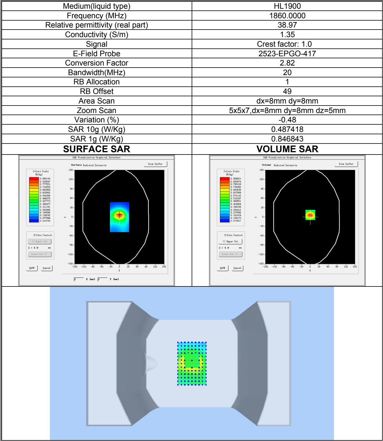
Plot 17:LTE BAND 2, Low channel (Body-worn, Back Side) Product Description:Smart Phone Test Date: 2025-12-01
