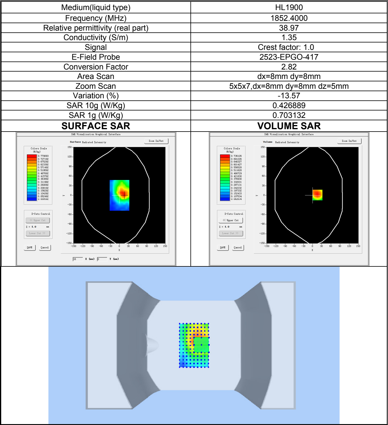
Plot 9: WCDMA BAND II, Low channel (Hotspot, Back Side) Product Description: Smart Phone Test Date: 2025-12-01
