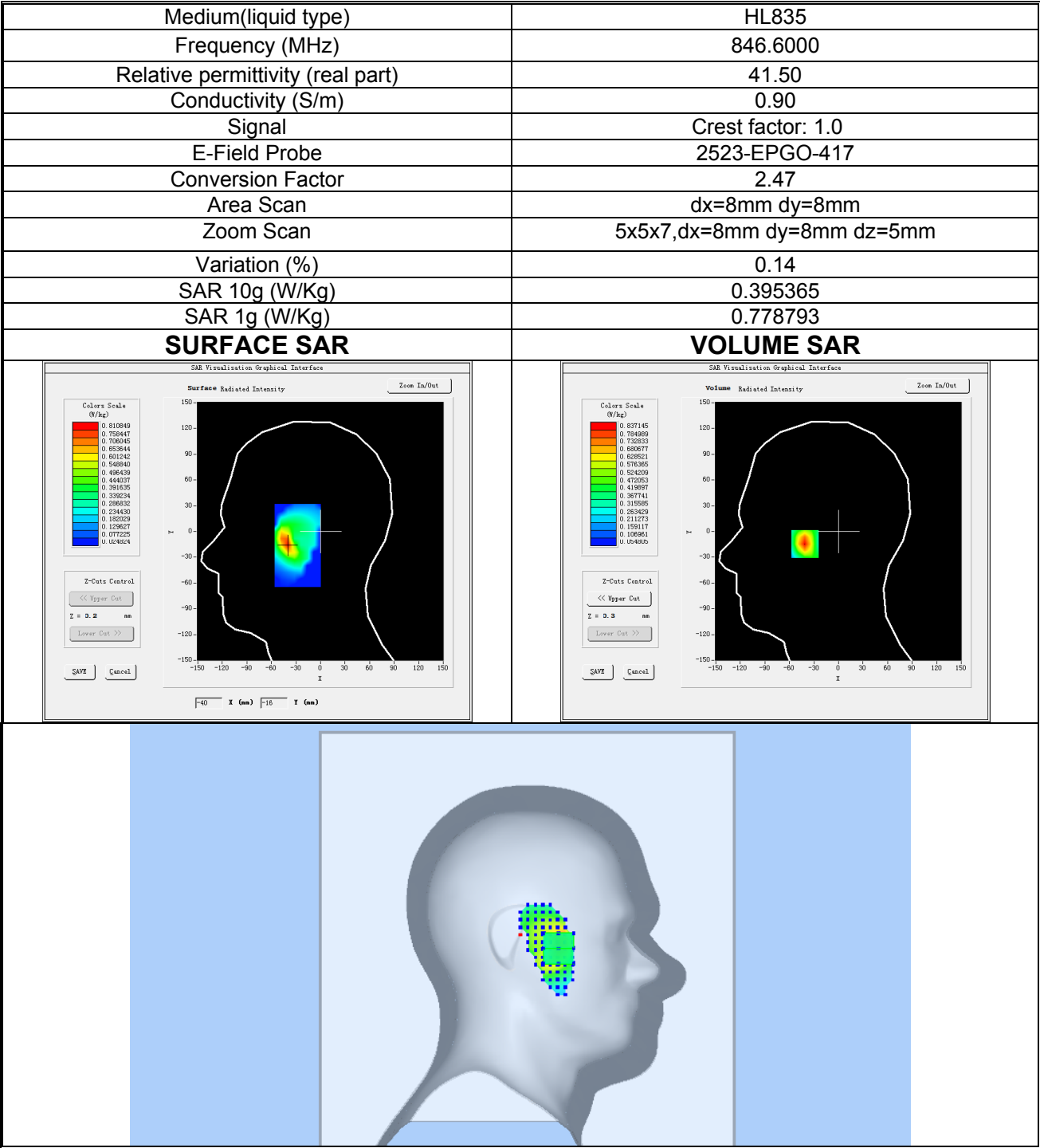
Plot 13: WCDMA BAND V, High channel (Left Head Cheek) Product Description: Smart Phone Test Date: 2025-12-02
