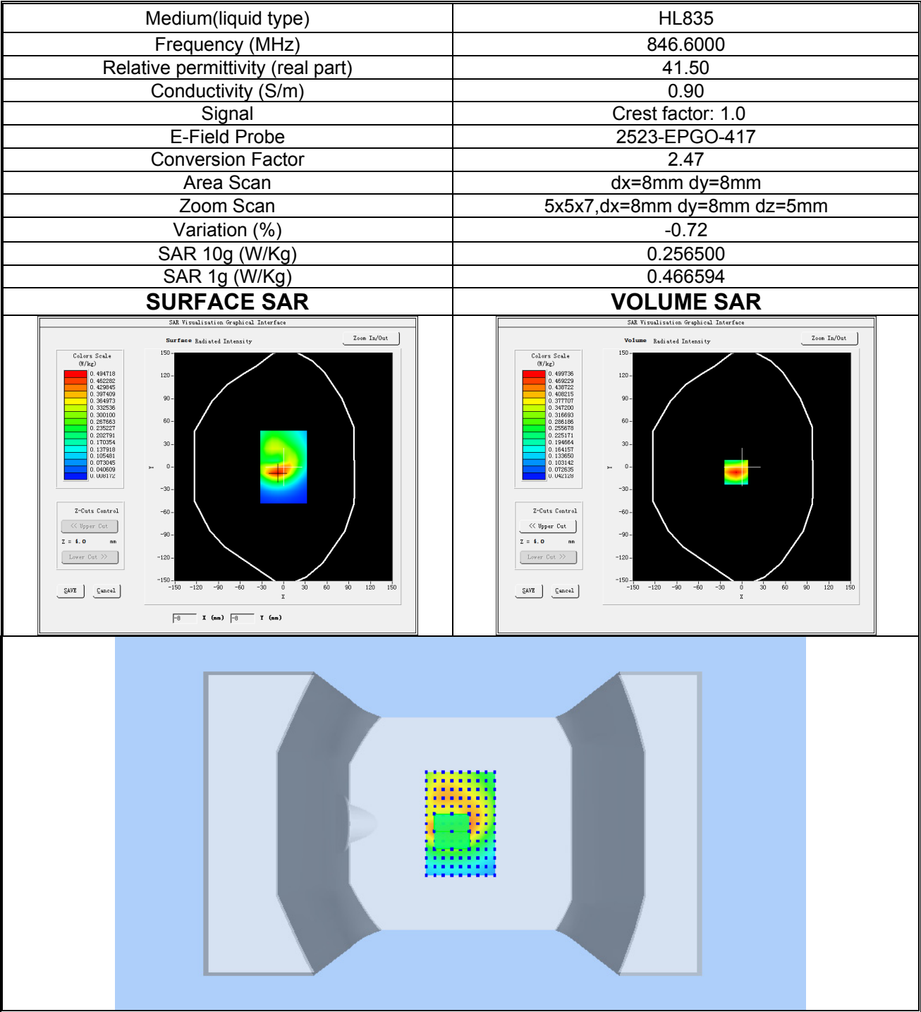
Plot 14: WCDMA BAND V, High channel (Body-worn, Back Side) Product Description: Smart Phone Test Date: 2025-12-02
