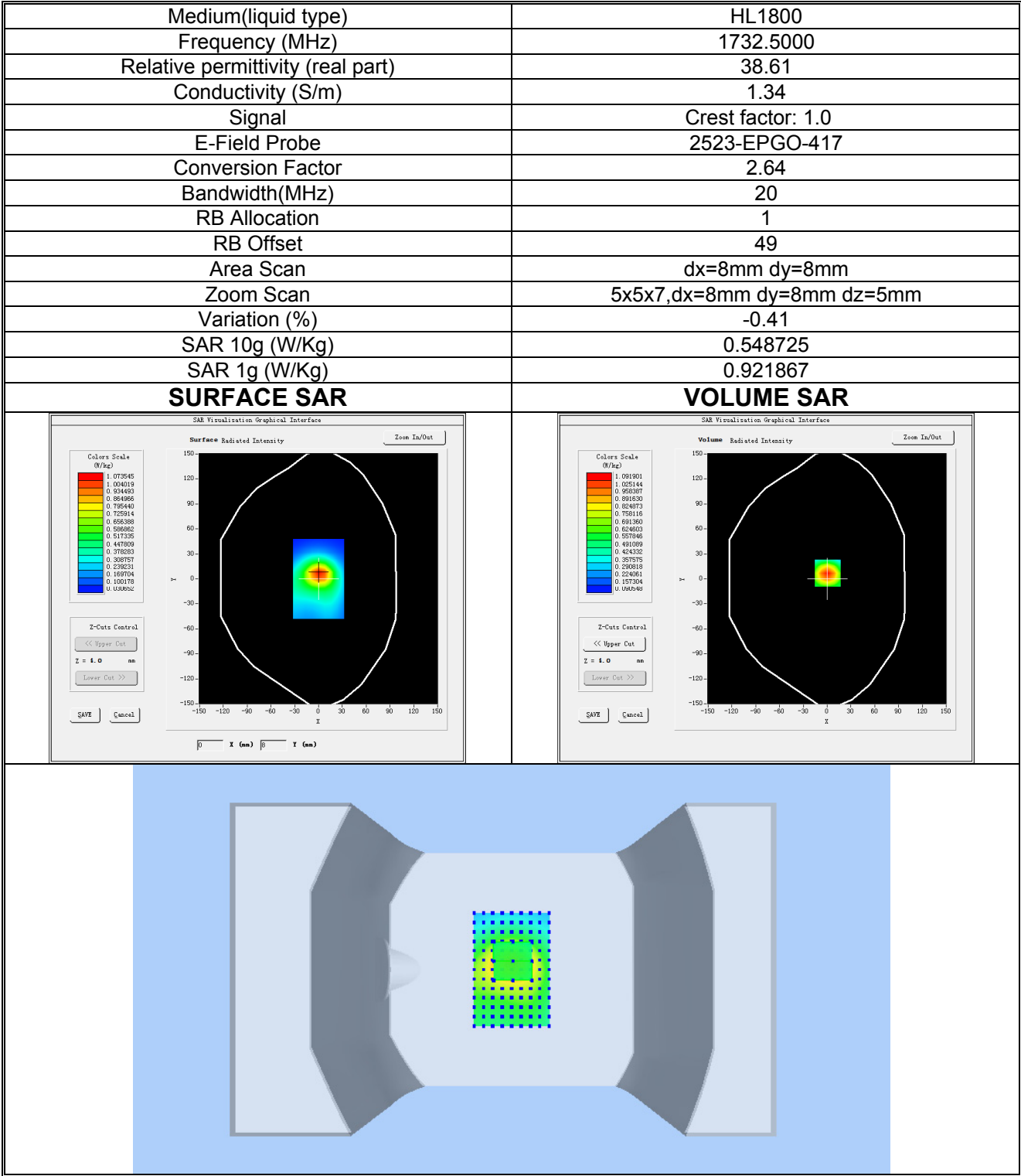
Plot 20: LTE BAND 4, Middle channel (Body-worn, Back Side) Product Description: Smart Phone Test Date: 2025-12-01
