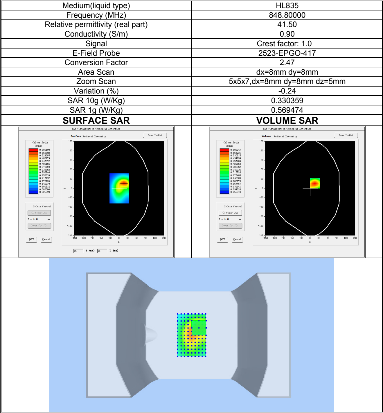
Plot 3: GPRS850, High channel (Hotspot, Back Side) Product Description:Smart Phone Test Date: 2025-12-02
