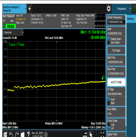
NTNV-N66-PC3-15-5-M-DFT-QPSK-Edge_1RB_R ight-3000-12000-Ant1-PASS
