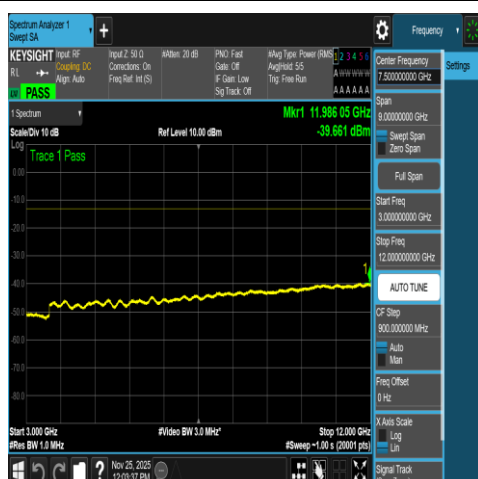
NTNV-N66-PC3-15-5-H-DFT-QPSK-Edge_1RB_R ight-3000-12000-Ant1-PASS
