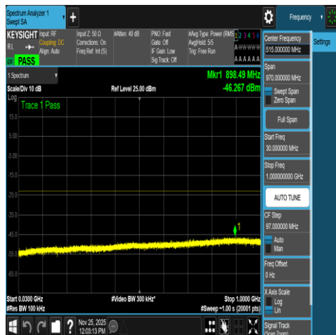
NTNV-N66-PC3-15-5-H-DFT-QPSK-Edge_1RB_R ight-30-1000-Ant1-PASS
