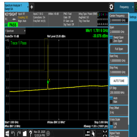
NTNV-N66-PC3-15-5-H-DFT-QPSK-Edge_1RB_R ight-1000-3000-Ant1-PASS
