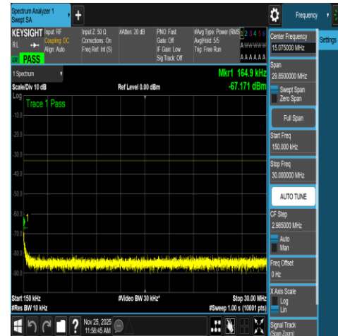
NTNV-N66-PC3-15-5-M-DFT-QPSK-Edge_1RB_R ight-0.15-30-Ant1-PASS
