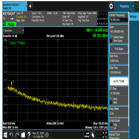
NTNV-N66-PC3-15-10-M-DFT-QPSK-Edge_1RB_ Left-0.009-0.15-Ant1-PASS
