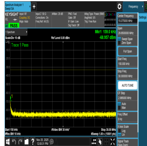
NTNV-N66-PC3-15-5-H-DFT-QPSK-Outter_Full-0. 15-30-Ant1-PASS
