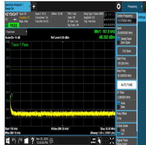
NTNV-N66-PC3-15-5-H-DFT-QPSK-Edge_1RB_R ight-0.15-30-Ant1-PASS
