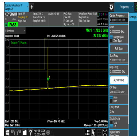
NTNV-N66-PC3-15-5-H-DFT-QPSK-Outter_Full-10 00-3000-Ant1-PASS
