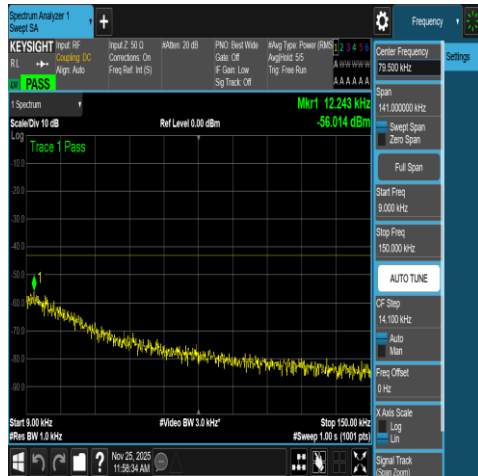
NTNV-N66-PC3-15-5-M-DFT-QPSK-Edge_1RB_R ight-0.009-0.15-Ant1-PASS
