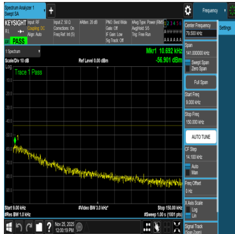
NTNV-N66-PC3-15-5-H-DFT-QPSK-Outter_Full-0. 009-0.15-Ant1-PASS
