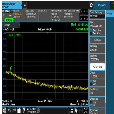
NTNV-N66-PC3-15-5-H-DFT-QPSK-Edge_1RB_R ight-0.009-0.15-Ant1-PASS
