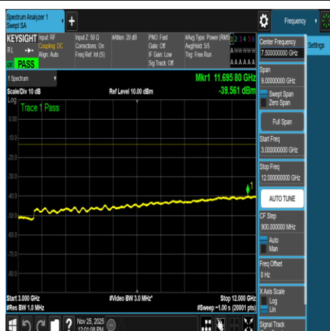
NTNV-N66-PC3-15-5-H-DFT-QPSK-Outter_Full-30 00-12000-Ant1-PASS
