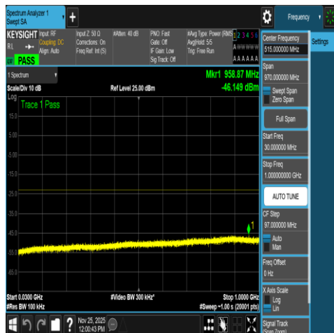
NTNV-N66-PC3-15-5-H-DFT-QPSK-Outter_Full-30 -1000-Ant1-PASS
