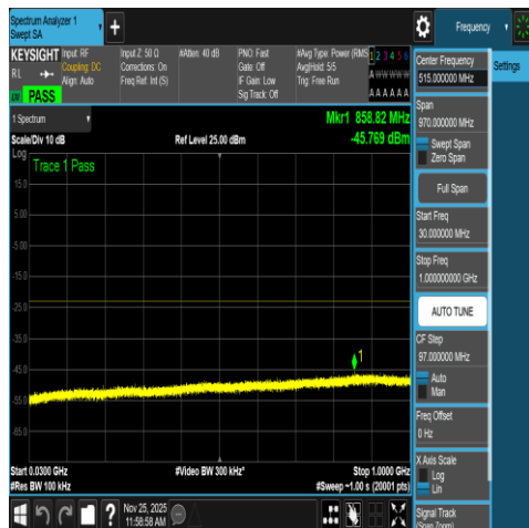
NTNV-N66-PC3-15-5-M-DFT-QPSK-Edge_1RB_R ight-30-1000-Ant1-PASS
