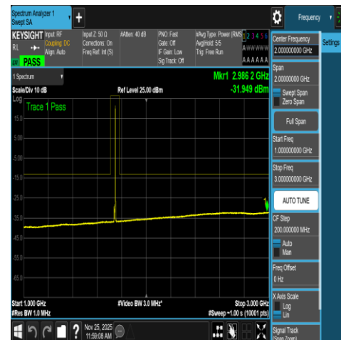
NTNV-N66-PC3-15-5-M-DFT-QPSK-Edge_1RB_R ight-1000-3000-Ant1-PASS
