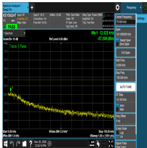
NTNV-N66-PC3-15-20-L-DFT-QPSK-Outter_Full-0. 009-0.15-Ant1-PASS
