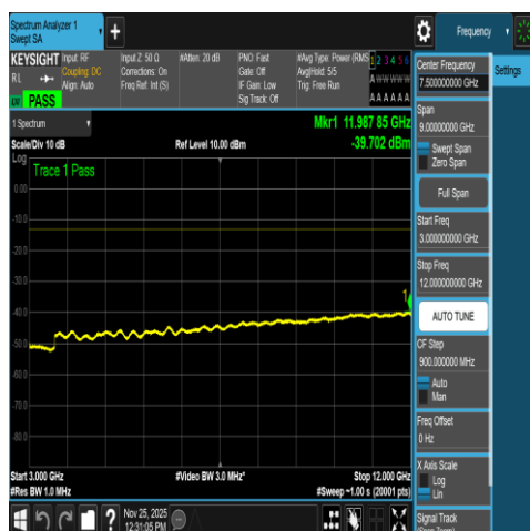
NTNV-N66-PC3-15-20-L-DFT-QPSK-Outter_Full-3 000-12000-Ant1-PASS
