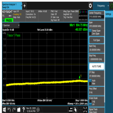
NTNV-N66-PC3-15-20-L-DFT-QPSK-Outter_Full-3 0-1000-Ant1-PASS
