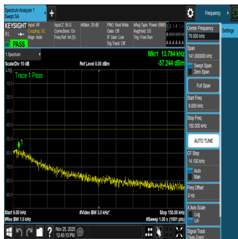
NTNV-N66-PC3-15-20-H-DFT-QPSK-Edge_1RB_ Left-0.009-0.15-Ant1-PASS
