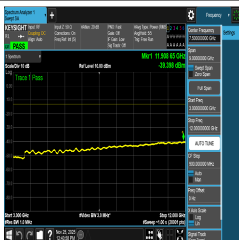
NTNV-N66-PC3-15-20-H-DFT-QPSK-Edge_1RB_ Left-3000-12000-Ant1-PASS
