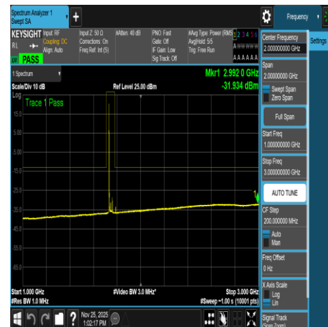
NTNV-N66-PC3-15-30-M-DFT-QPSK-Edge_1RB_ Left-1000-3000-Ant1-PASS
