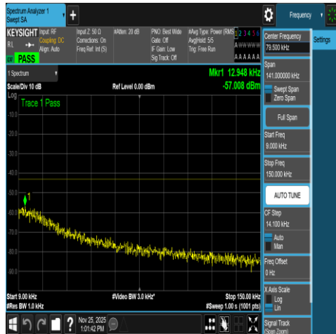
NTNV-N66-PC3-15-30-M-DFT-QPSK-Edge_1RB_ Left-0.009-0.15-Ant1-PASS
