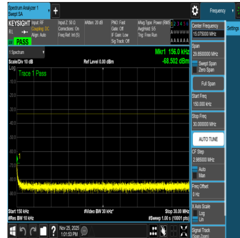
NTNV-N66-PC3-15-30-M-DFT-QPSK-Edge_1RB_ Left-0.15-30-Ant1-PASS
