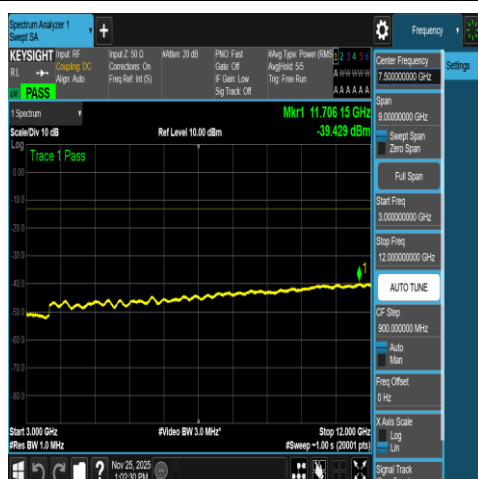
NTNV-N66-PC3-15-30-M-DFT-QPSK-Edge_1RB_ Left-3000-12000-Ant1-PASS
